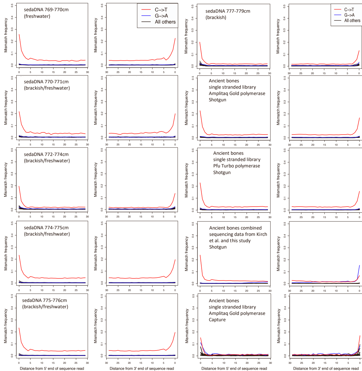
Figure S1. Post-mortem deamination patterns for filtered reads sequenced from the Late Pleistocene sedaDNA samples and stickleback bones, mapped against the threespine stickleback reference genome gasAcu1.0, Related to Figure 2. Sequence misincorporation errors at the 5' read termini of sequence data show characteristic (C>T) post-mortem damage patterns relative to the modern stickleback reference (gasAcu1). Sequence misincorporation errors at the 3' read termini of sequence data show characteristic (C>T) post-mortem damage patterns in single-stranded libraries and the reverse complement (G>A) in double-stranded libraries.
