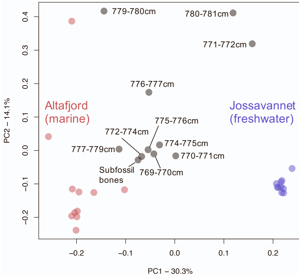
Figure S2. Principal component analyses (PCA) of Late Pleistocene and contemporary stickleback genomes from Finnmark, Norway, Related to Figure 3. Principal component analyses (PCA) of 14,075 transversions in marine-freshwater divergent regions of the stickleback genome. Colored markers represent genomes sampled from present-day stickleback populations at Jossavannet freshwater lake (blue markers) and the adjacent (marine) Altafjord (red markers), and Late Pleistocene (~12.9 kyr-old) genomes recovered from subfossil bones or sediment at Jossavannet (black markers). The depth of each sediment layer is given in the marker labels. The variation in coverage of marine-freshwater regions, which will include loci of different effect size, biases comparisons between sediment layers.
