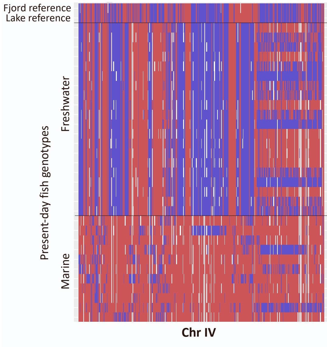
Figure S3. Comparison of mapping biases due to reference marine or freshwater reference genome, Related to Figure 3. Visual genotypes at 465 transversions in the marine-freshwater divergent regions of chromosome IV for contemporary Jossavannet (freshwater) and Altafjord (marine) sticklebacks, and an ancient environmental genome from freshwater sediment layer (769-770 cm depth, top two rows). The lower of these two rows is based on mapping sequence data to the gasAcu1.0 reference assembly generated from a Pacific freshwater sample from Bear Paw Lake, Alaska S1 . The top row is mapped to an alternative reference generated by mapping a modern fjord sample to the gasAcu1.0 and generating a haploid fasta file. There is some missingness of data, but the overall patterns of freshwater and marine alleles is consistent between the two mapping references. Rows are individual fish, columns are sites, which are shaded red for the most common allele in the marine population, blue for the alternative allele, and white for missing data.
