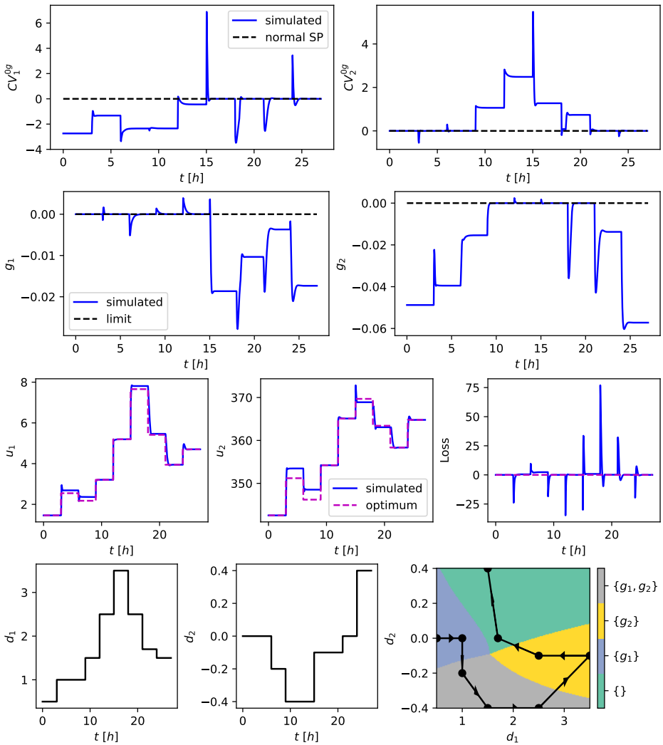
Figure 2.11: Closed-loop simulation results for case study 2.
