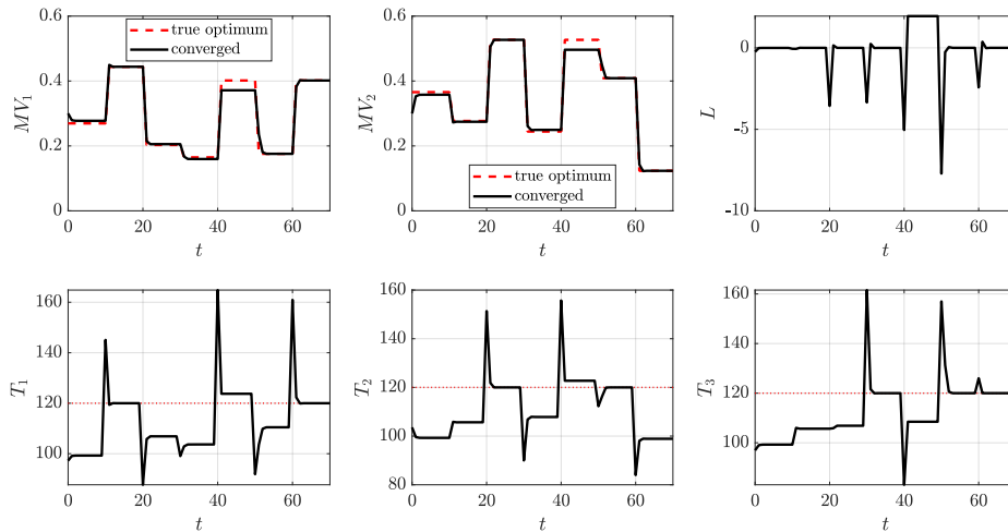
Figure 5.4: Simulation of steady-state RTO with model-plant mismatch
