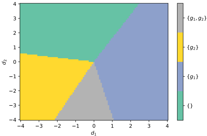
Figure 2.5: Active constraint regions for case study 1 as a function of disturbances.
