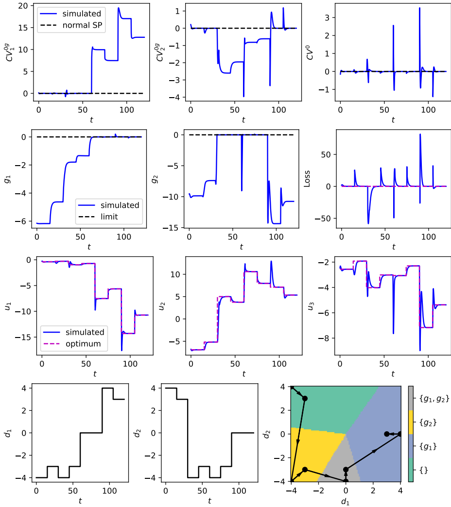
Figure 2.7: Closed-loop simulation results for case study 1.
