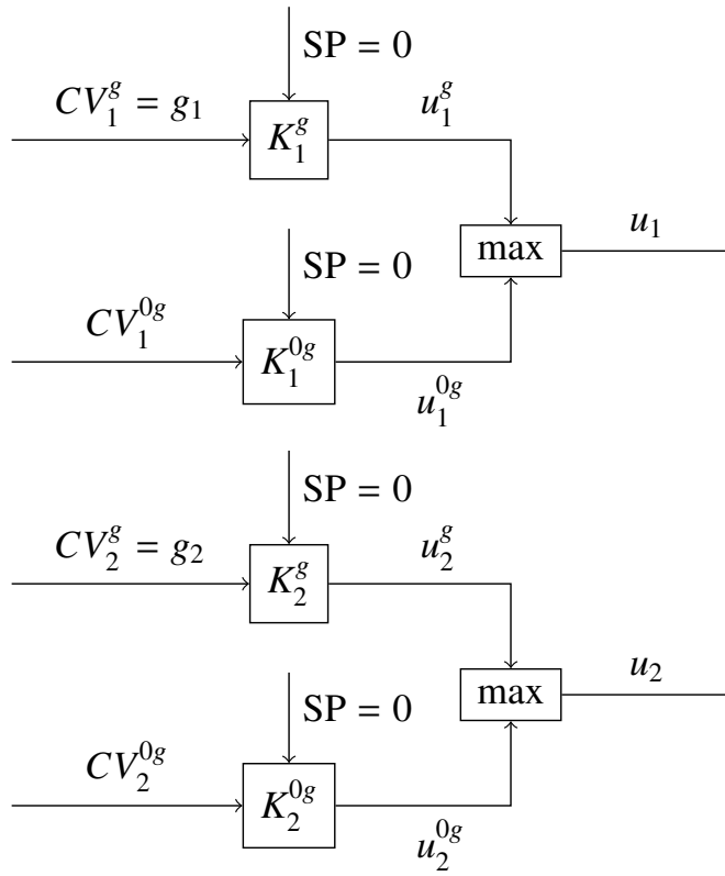
Figure 2.10: Complete control structure for case study 2.
