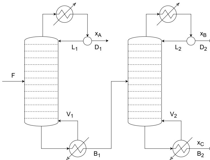
Figure 6.8: Scheme of two distillation columns in sequence, based on Jacobsen and Skogstad (2012)
