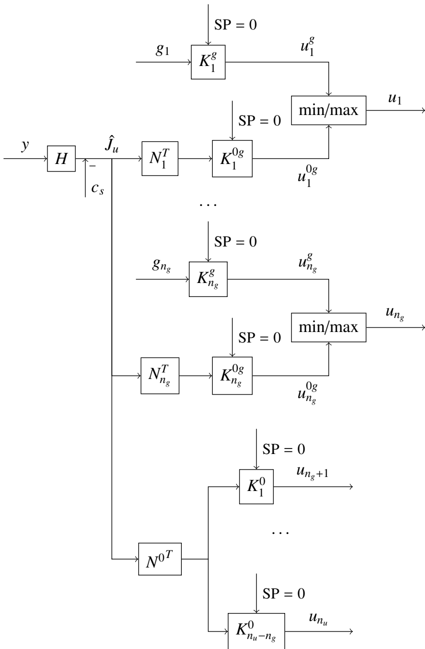
Figure 4.4: Decentralized region-based optimizing control structure using SISO controllers and selectors.
