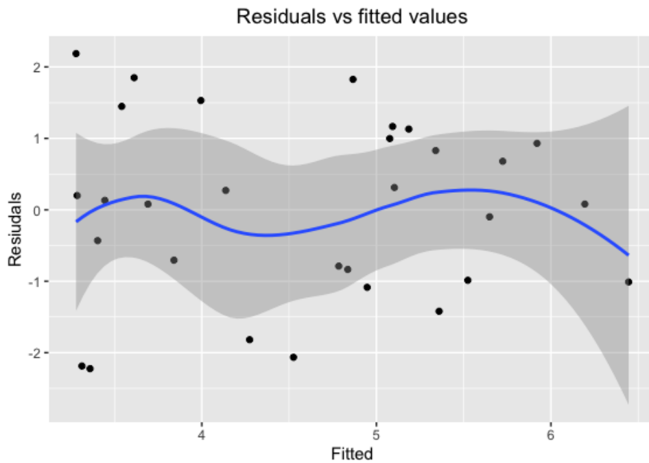
Figure 5.2: Residuals vs fitted values
