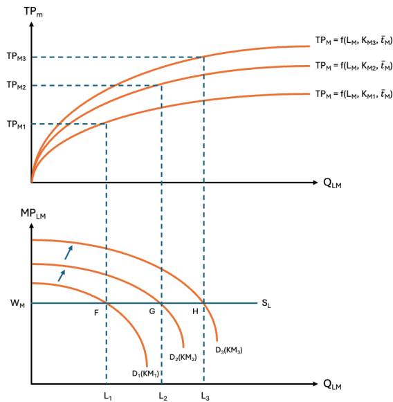
Figure 3.3: An overview of the effect of shifts in the Lewis model.
