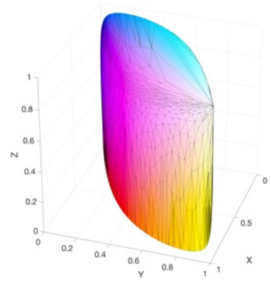
(c) Optimised spherical sampling. 1051 unique vertices.
