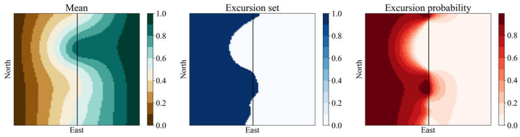
(a) Updated predictive field based on empirical data from ground truth scenario I.
