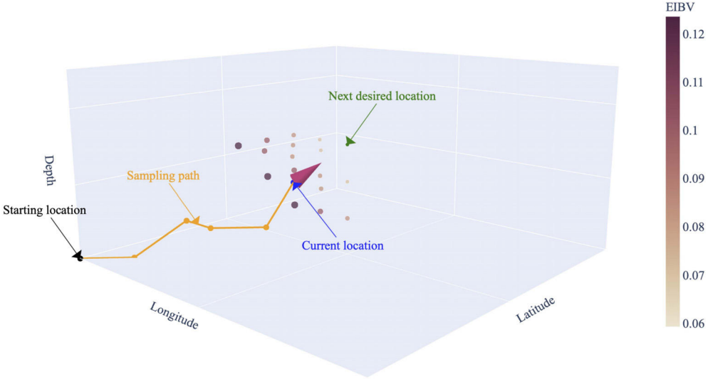
Fig. 2. Adaptive path example on a 3-D waypoint graph. There are 17 candidate locations in different layers, the blue dot shows the current AUV location whereas the green dot indicates the desired next waypoint selected based on the minimum EIBV criterion.
