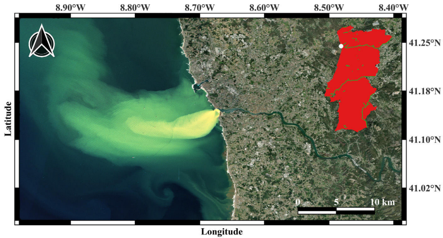
Figure 2.1: Sentinel-2 image of the Douro River plume. Captured on 5 January 2020. Courtesy of Copernicus Open Access Hub.
