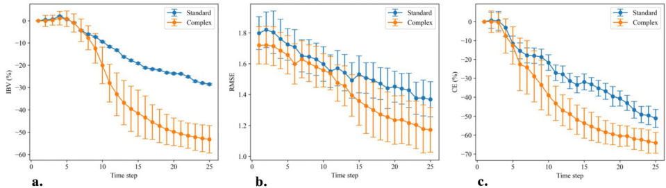
Fig. 8: Variation in integrated Bernoulli variance (a), root mean square error (b), and classification error (c) over the 100 replicate runs with the standard model (blue) and the complex model (orange). The solid lines show the averages and the vertical errorbars show the empirical standard deviations of the respective metrics.
