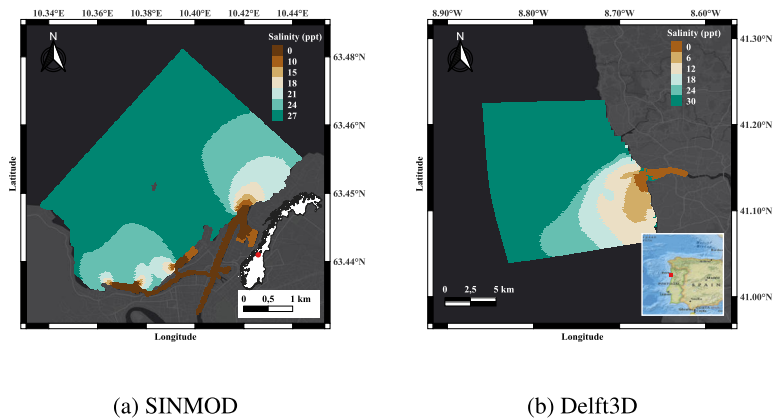
Figure 2.4: Comparison of surface salinity estimates from SINMOD and Delft3D in the Trondheimsfjord and Rio Douro regions.
