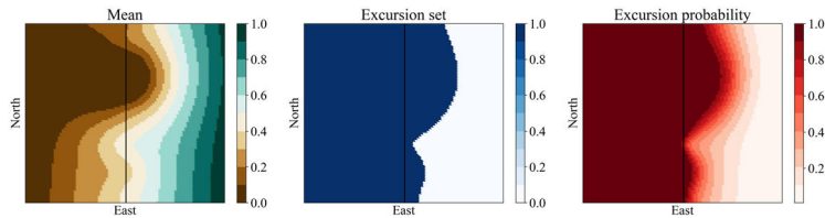
(c) Updated predictive field based on empirical data from ground truth scenario III.
