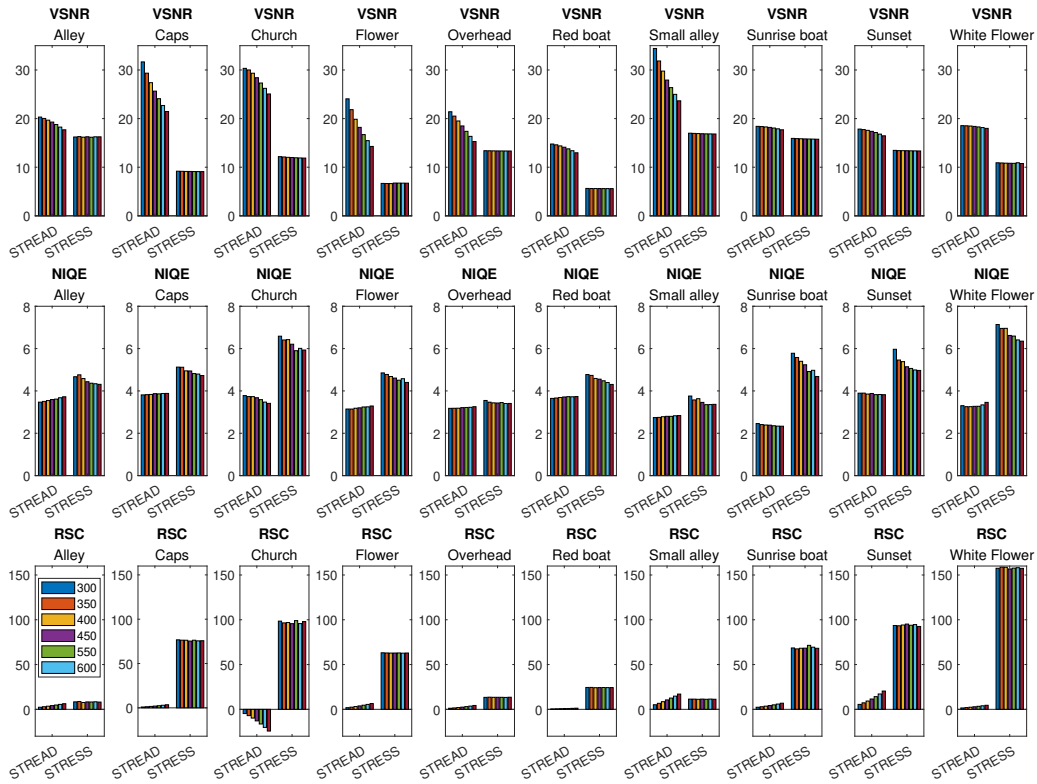
Figure 16: VSNR (top), NIQE (middle) and RSC (bottom) for the 10 images. For VSNR higher values are better, for NIQE lower values are better, while for RSC higher values indicate higher contrast than the original. We can see that for VSNR and NIQE the proposed STREAD in all images has better values compared to STRESS. For 9 out of the 10 images, STREAD produces images with higher contrast. Colour in the legend indicates the number of iterations.
