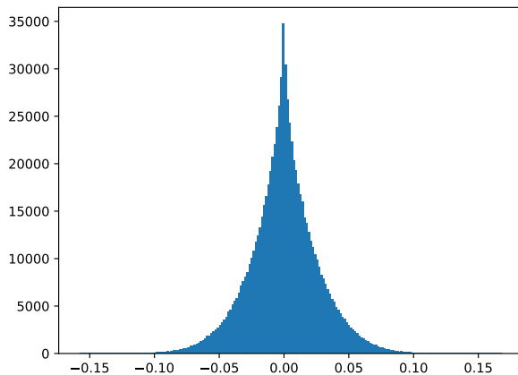
Figure 1: Histogram of the noised caused by the random sampling in the STRESS algorithm.
