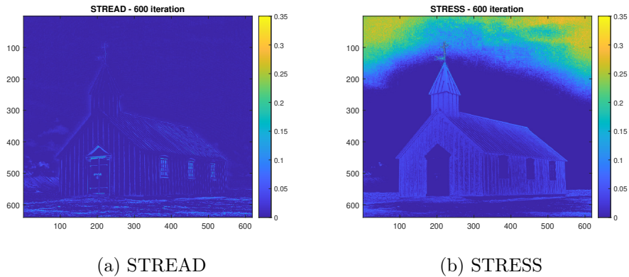
Figure 17: The difference between the original and enhanced images for each pixel for the church image, with 600 iterations for each method.
