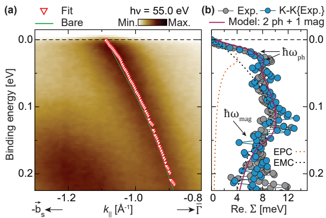
FIG. 2. Electron-boson coupling (EBC) in the spin minority band along -\mathbf{b}_s near the high-symmetry points \bar{M} and \bar{K} . (a): The measured energy bandstructure, overlaid with the unrenormalized (green) band and the experimentally determined, renormalized spin band position (red triangles). (b): The real self-energy \text{Re } \Sigma of the fitted band in (a). The \text{Re } \Sigma (gray) found from Eq. 2 is shown to satisfy causality with \text{Im } \Sigma through the Kramers-Kronig transformation (blue). A three-boson model (purple line) consisting of two distinct electron-phonon couplings (EPCs) with energies \hbar\omega_{\text{ph}} = 18 meV and \hbar\omega_{\text{ph}} = 36 meV, respectively, and one electron-magnon coupling (EMC) with energy \hbar\omega_{\text{mag}} = 154 meV, best describes the measured line shape. The individual EPC (dashed orange) and EMC (dashed black) models are highlighted.
