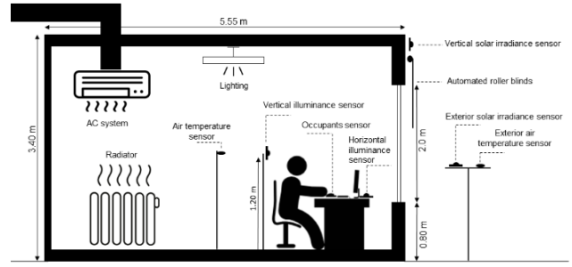
Figure 2: Schematic presentation of sensor placements under the ISO 52016-3-recommended control method. (Norouzasas, Tabadkani, et al., 2023)
