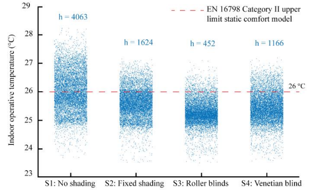
Figure 4: Distribution of indoor operative temperature for each scenario according to EN16798 category II.
