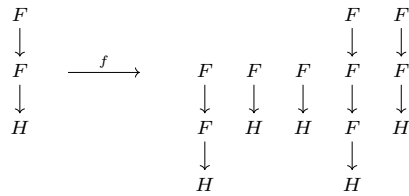
Fig. 15. Attaching a single representation cell.
