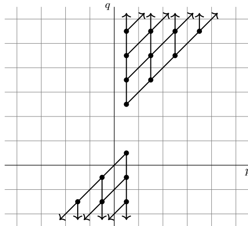
Fig. 3. The cohomology of H(2) .
