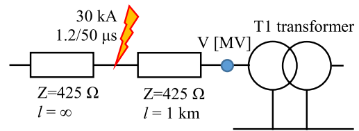
Fig. 14. Simulation of lightning overvoltages using the T1 transformer models. Open transformer secondary, M2 with disconnected inductance.
