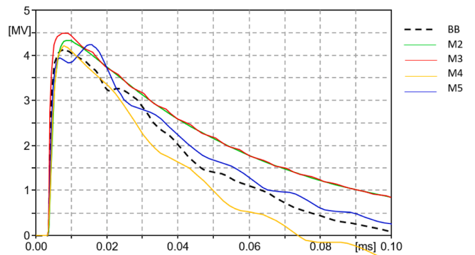
Fig. 15. Simulated lightning overvoltage at transformer terminal using the T1 test-report transformer models from Fig. 8.
