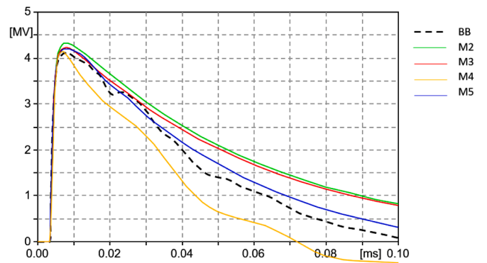
Fig. 16. Simulated lightning overvoltage at transformer terminal using the T1 fitted transformer models from Fig. 10.
