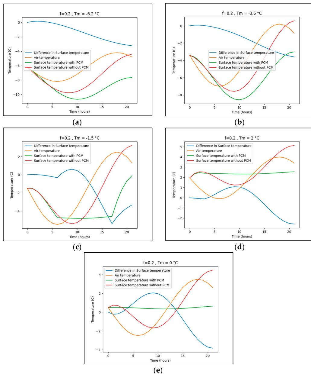
Figure A1. The effect of PCMs on the surface temperature of the pavement. (a) Trondheim. (b) Beijing. (c) Zanjan. (d) Berlin. (e) NY.
