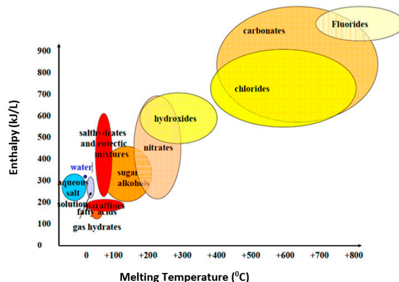
Figure 3. Melting point vs. heat storage capacity of various PCMs reprinted/adapted from Ref. [74,76].
