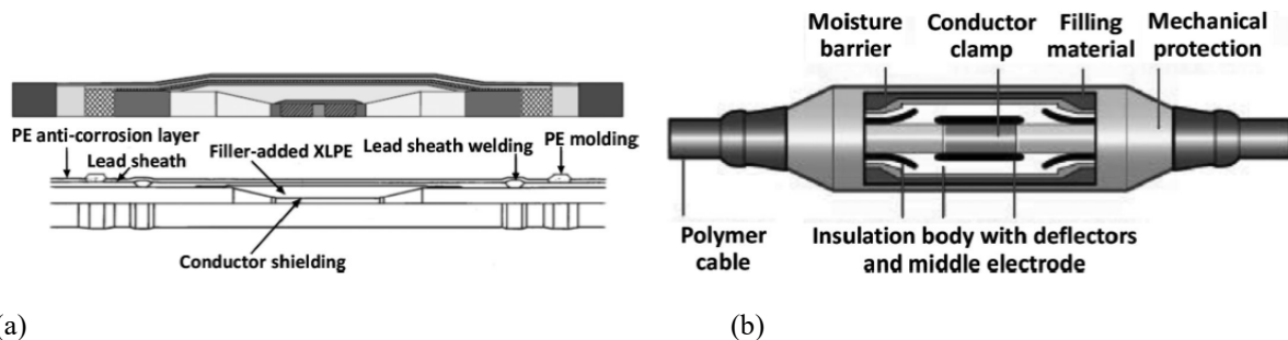
Figure 2. (a) Factory joint for HVDC submarine cable and (b) pre-molded joint for HVDC land cable, after [4, 10].
