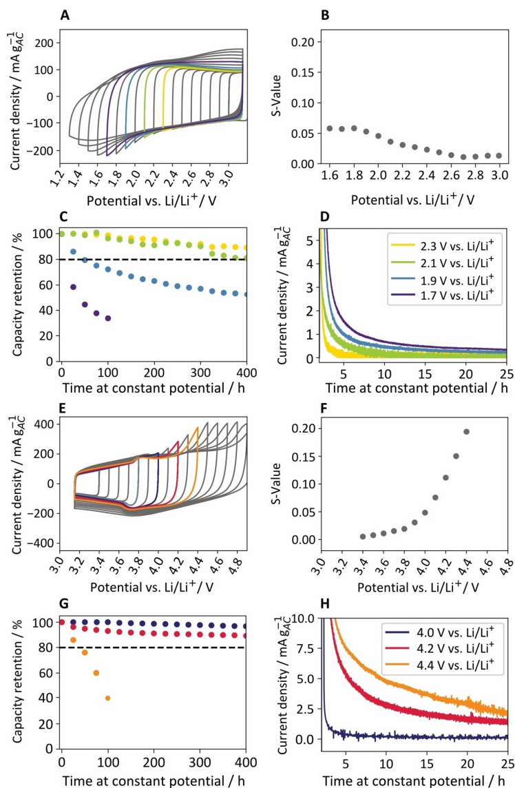
Figure 7. Cathodic and anodic stability of \text{LiPF}_6 on AC in three-electrode half-cell setup. A, E) Cyclic voltammograms with gradual lowering (increase) of vertex potential. B, F) S-value extracted from negative (positive) CVs. C, G) Capacity retention during voltage hold tests at selected negative (positive) potentials. D, H) Leakage currents during first 25 h of voltage hold test at negative (positive) potentials.
