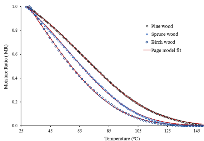
Fig. 2. Experimental and predicted (Page model) moisture ratios for pine, spruce, and birch wood at 30 K/min.
