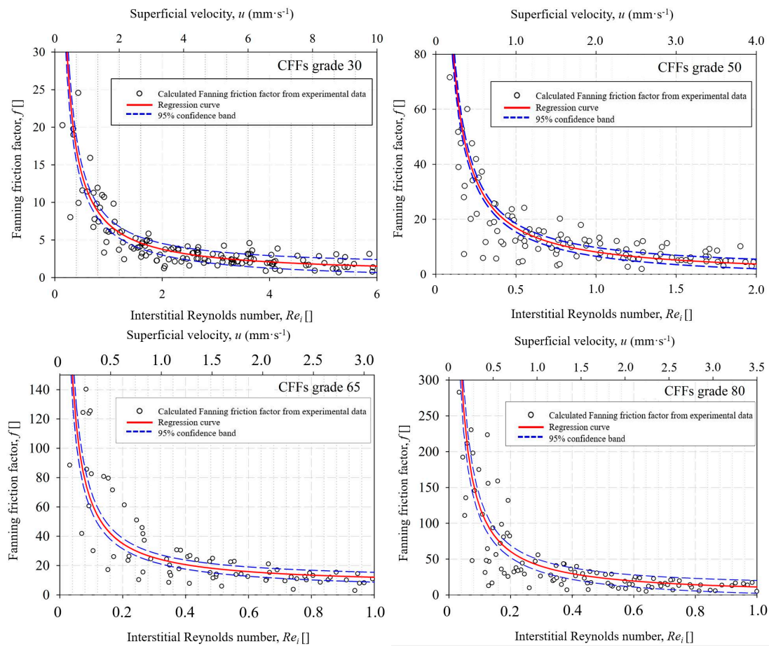
Figure 9. The Fanning friction factor (dimensionless) as a function of the interstitial Reynolds numbers ( Re_i ) and superficial velocity ( u ) for CFFs Grade 30–80 from supplier A.
