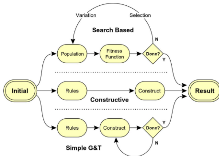
Figure 3.2: Procedural Content Generation Methods
