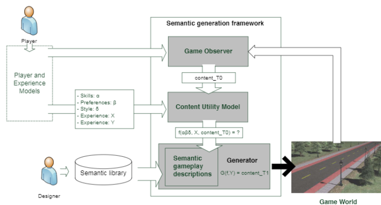
Figure 4.1: Generation framework [23]
