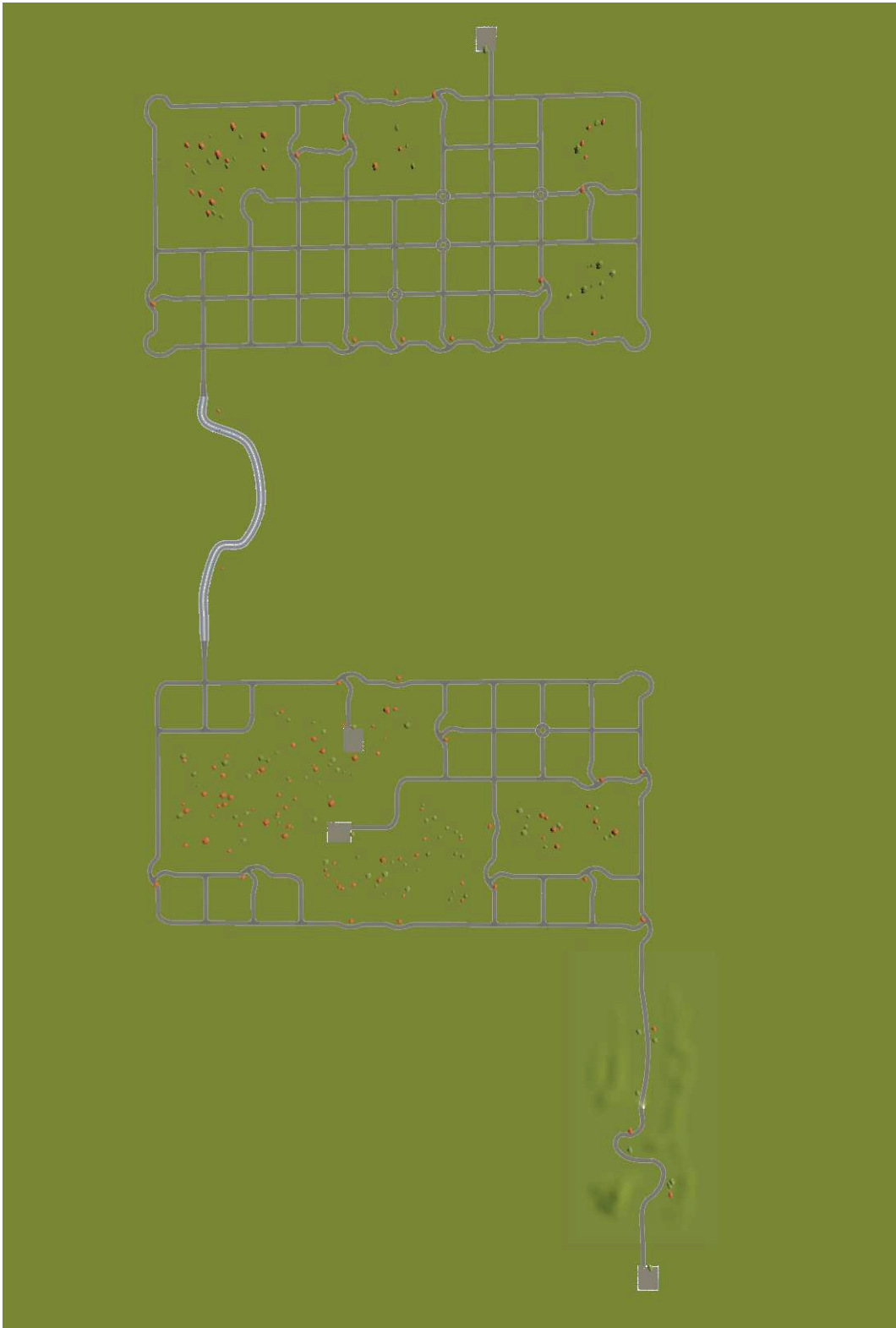
Figure 5.6: Generated lesson
