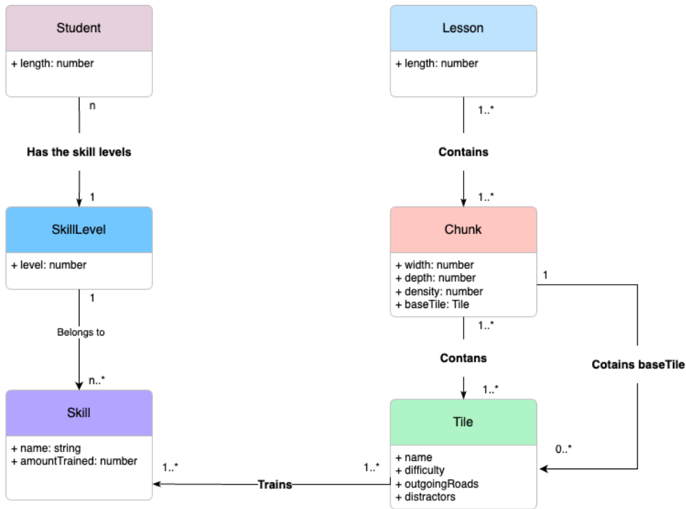
Figure 5.2: Class diagram
