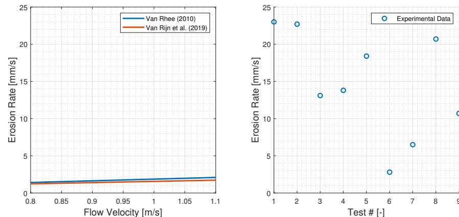
Figure 12. Comparison between estimated (left) and real erosion rates (right). For comparison's sake, y-axis has the same limits in the two sub-figures (Van Rhee [22] and Van Rijn et al. [23]).
