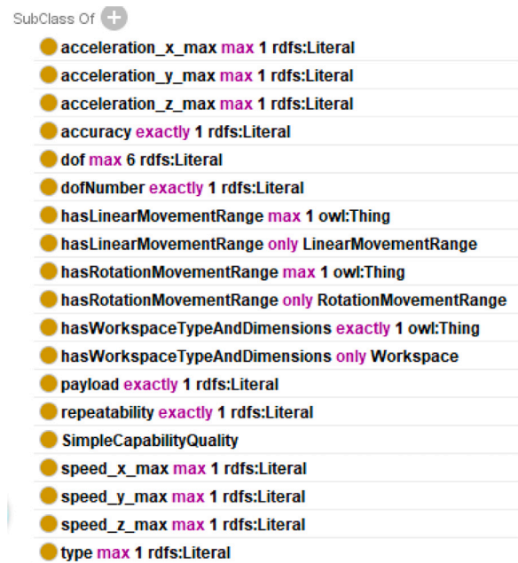
Fig. 6. Property restrictions defined for the “Moving” Capability as visualised from Protege ontology editor, vocabulary from [62].
