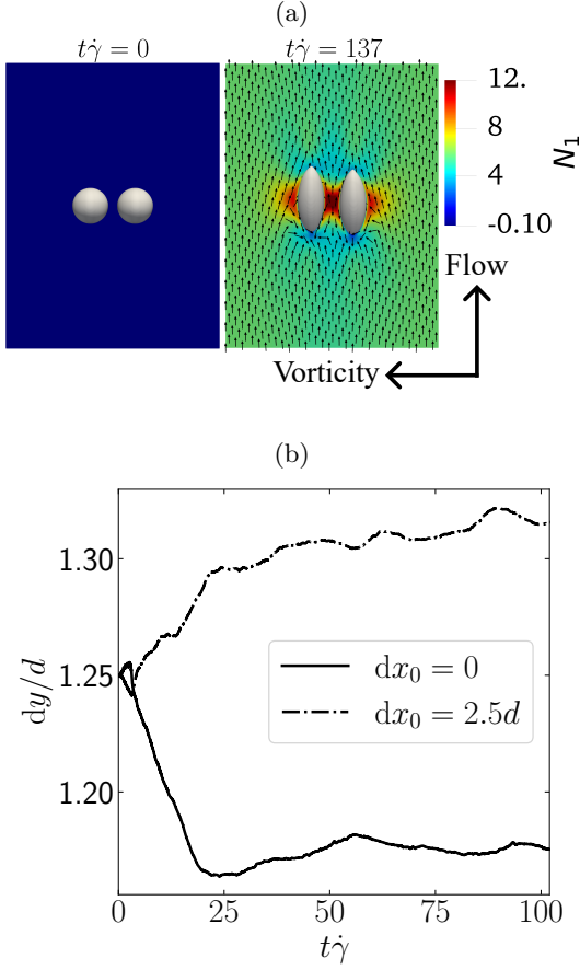
FIG. 12: Average relative position in the vorticity direction as a function of time for two dx_0 in Emulsion Em3, simulated with the EVP model with Re = 0.05 , Ca = 0.5 , Wi = 7.023 , \alpha_s = 1./9 , Bn = 0.422 , n = 0.5 , dy_0 = 1.25d .
