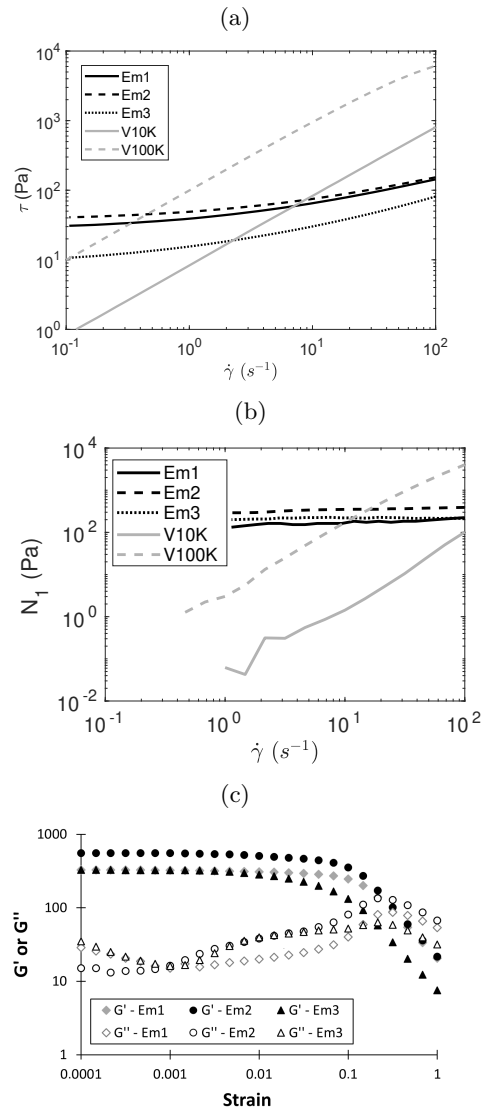
FIG. 2: Rheological properties of the fluids used in the experiments. (a) Viscous shear stress \tau measured by a shear rate ramp. (b) First normal stress difference. In the emulsions (Em1, Em2, Em3), N_1 has been measured in a shear rate ramp. In the silicone oils (V10K, V100K), it has been deduced from oscillation tests at angular frequency \omega using the empirical rule N_1(\dot{\gamma}) \simeq 2G'(\omega) [29]. (c) Elastic ( G' ) and viscous ( G'' ) moduli of the emulsions measured by strain amplitude sweep with oscillation at angular frequency 6.3 rad/s.
