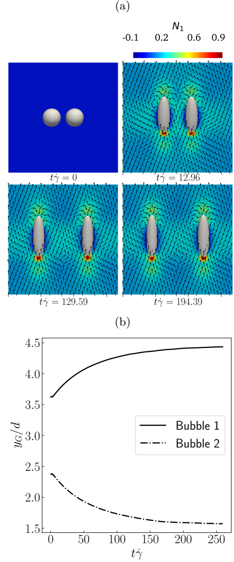
FIG. 14: Motion of bubble-pair suspended in a weakly VE silicone oil when they are initially aligned in the vorticity direction. (a) Visualisation of the evolution of the bubble-oil interface at four snapshots in time, as well as the N_1 contours and streamlines on the central XY plane. (b) COM positions of bubbles 1 and 2 in the vorticity direction as a function of time. Bubble 1 corresponds to the right bubble in each snapshot, and Bubble 2 the left. Re = 0.05 , Ca = 0.5 , Wi = 0.1 , initial separation distance of the COM of the bubbles: dx_0 = 0 , dy_0 = 1.25d .
