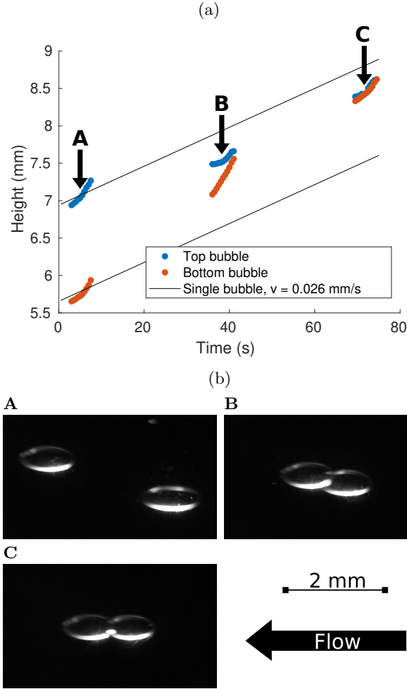
FIG. 6: (a) Two bubbles in EM2 interacting in shear flow, where the position of the center of mass of each bubble is tracked in time. The black lines indicate the trajectories of the bubbles if they did not interact. (b) Pictures of the bubbles at three different times indicated by the arrows are shown to illustrate the chaining process.
