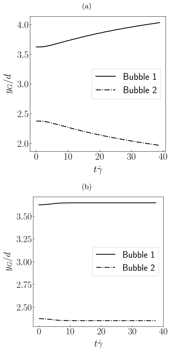
FIG. 17: Trajectory of the COM position in the vorticity direction for a bubble-pair initially aligned in the vorticity direction in a Newtonian suspending phase for Re = 0.05 and (a) Ca = 0.5 , (b) Ca = 0.05 . The initial configuration of the bubbles, and their indexing (i.e., Bubble 1 and 2), are as in Fig. 14.
