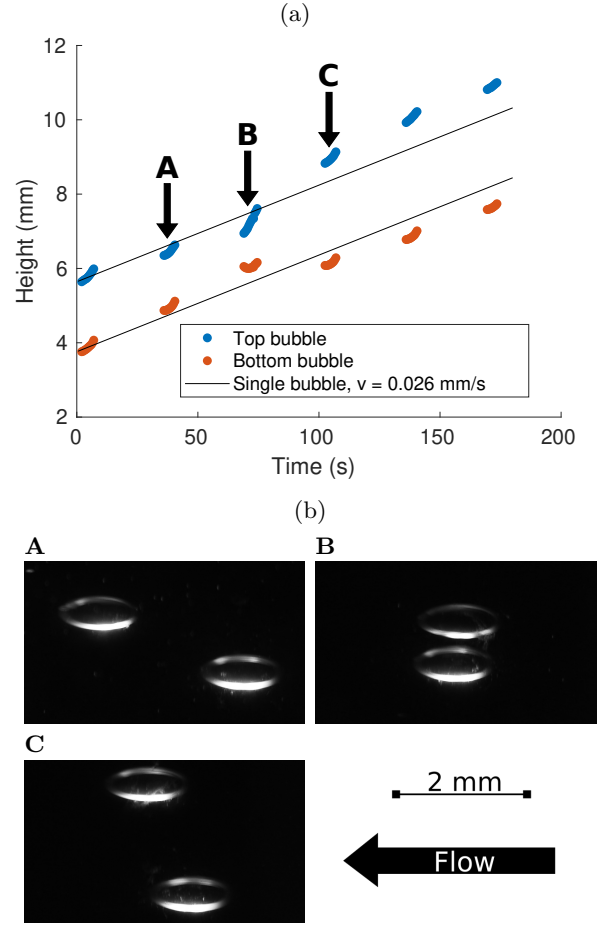
FIG. 7: (a) Repulsion between two bubbles in Em2 in shear flow, where we track their center of mass with time. The black lines indicate the trajectories of the bubbles if they did not interact. Initially, the bubbles are not aligned in the vorticity direction and attract each other (arrow A). As soon as they become aligned in the vorticity direction (arrow B), they repel each other. (b) A-C show three images at different times as the bubble repel each other.
