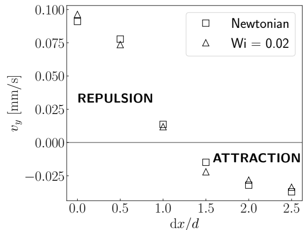
FIG. 15: Migration velocity of the bubble-pair in Newtonian suspending phase, and weakly VE silicone oil suspending phase as a function of the bubble separation distance in the flow direction. Re = 0.05 , Ca = 0.5 , dy/d = 2 .
