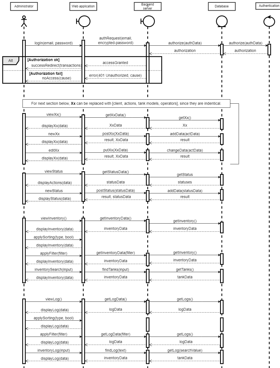
Figure 3.3: Sequence diagram showing how the different components of the web app cooperates
