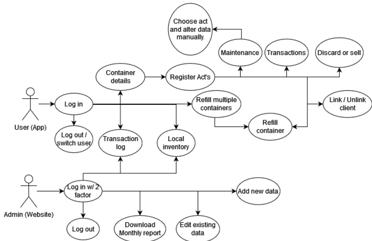
Fig 1: Use case model
