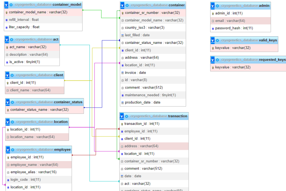
Figure 5.2: A visual representation of the database structure.
