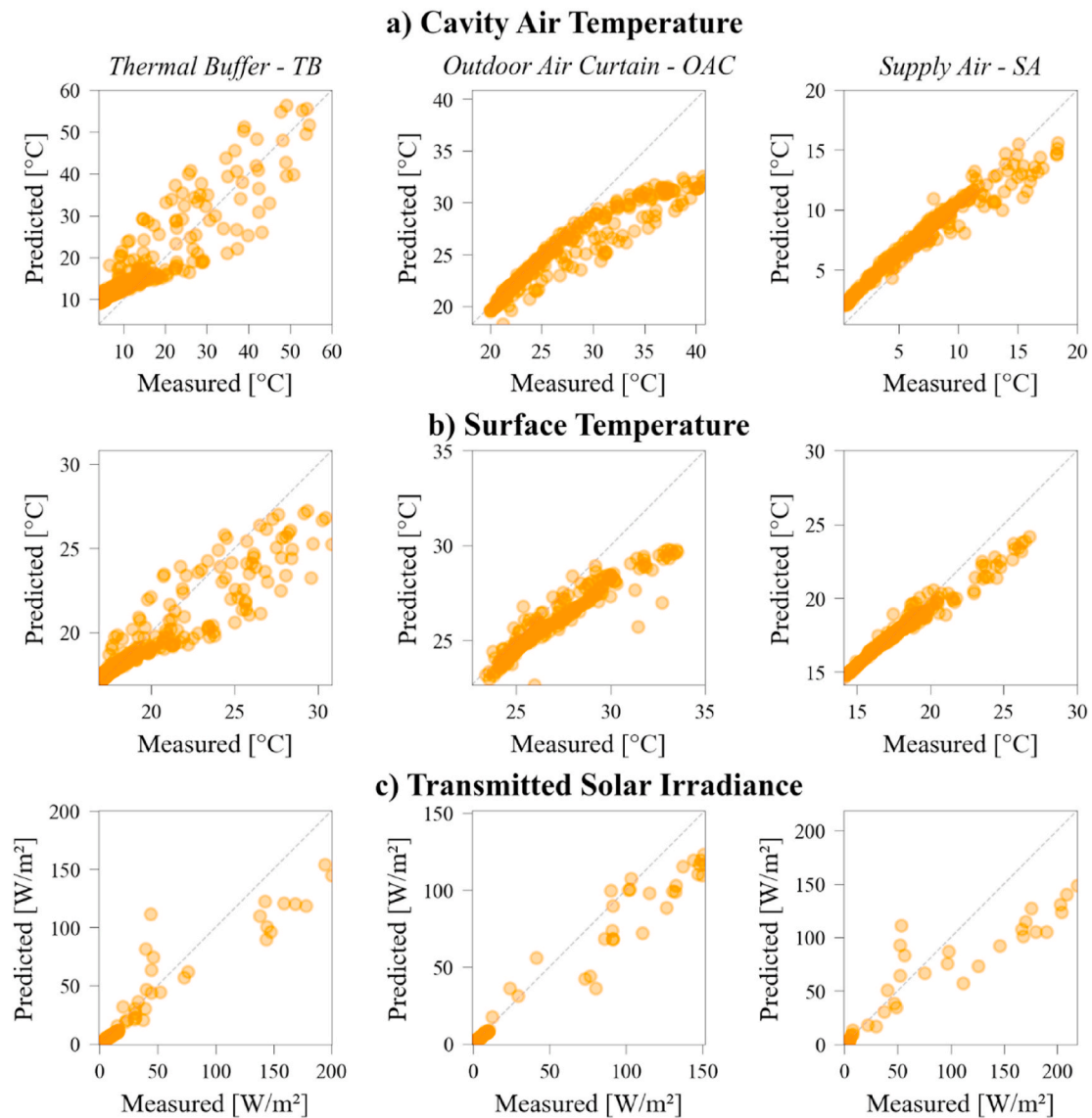
Fig. 8. Comparison between experimental data and predicted outcomes carried out with IES-VE. From top to bottom: Cavity air temperature, Surface Temperature, Transmitted Solar Irradiance. From left to right: Thermal Buffer, Outdoor Air Curtain and Supply Air. The shading configurations are combined.
