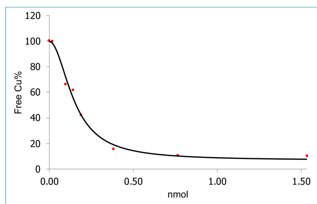
FIGURE 7 Curve fitting using a 4PL symmetrical sigmoidal plot, X = 0.16 nmol at 50% bound, R 2 = 0.9892,
