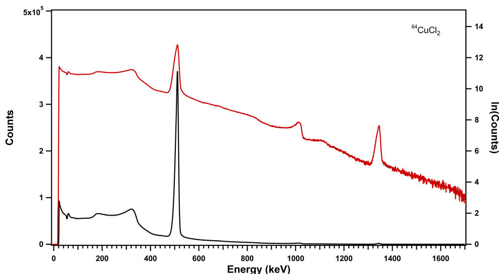
FIGURE 3 HPGe analysis of the cyclotron produced copper-64 after purification in the Alceo setup
