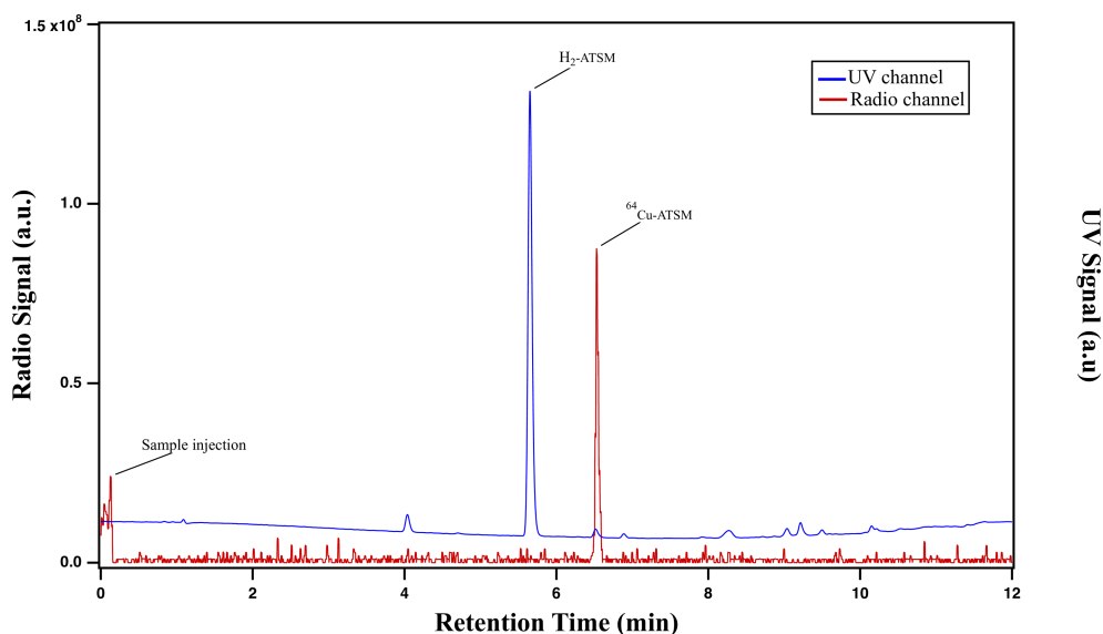
FIGURE 5 UV signal and radio signal of the finished product on HPLC
