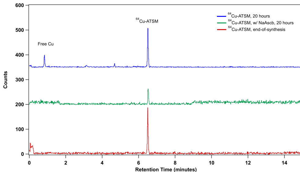
FIGURE 8 Radio HPLC analysis of the product and the decayed product after 20 h with and without sodium ascorbate formulation.
