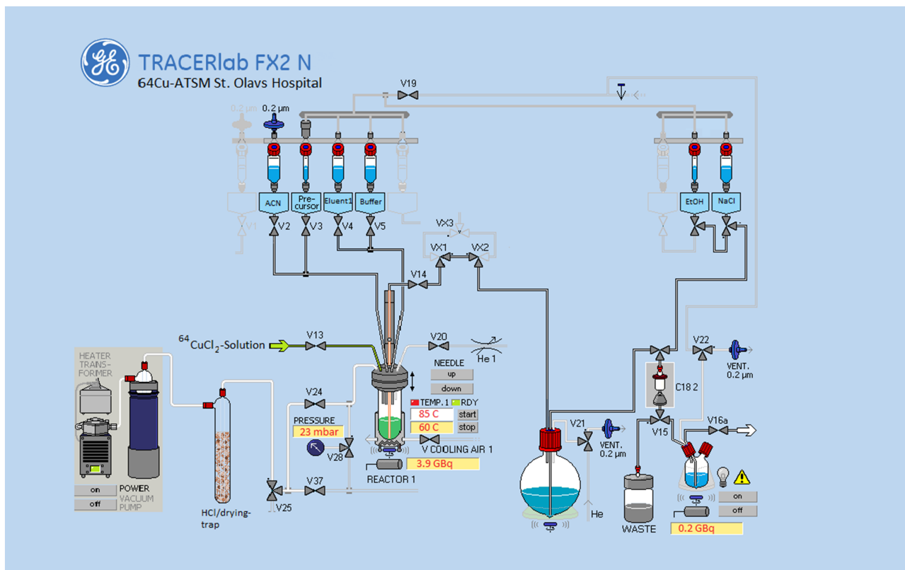
FIGURE 2 ^{64}\text{Cu} -ATSM production layout on the Tracerlab FX2 N
