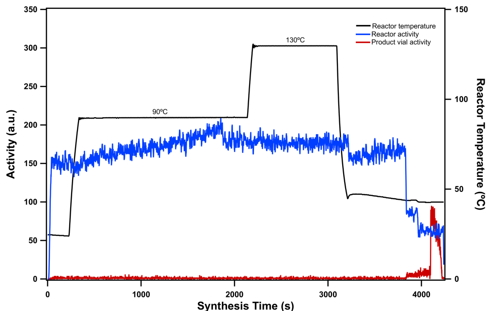
FIGURE 9 Tracerlab FX2 N report showing the heat profile and activity over the course of the synthesis run
