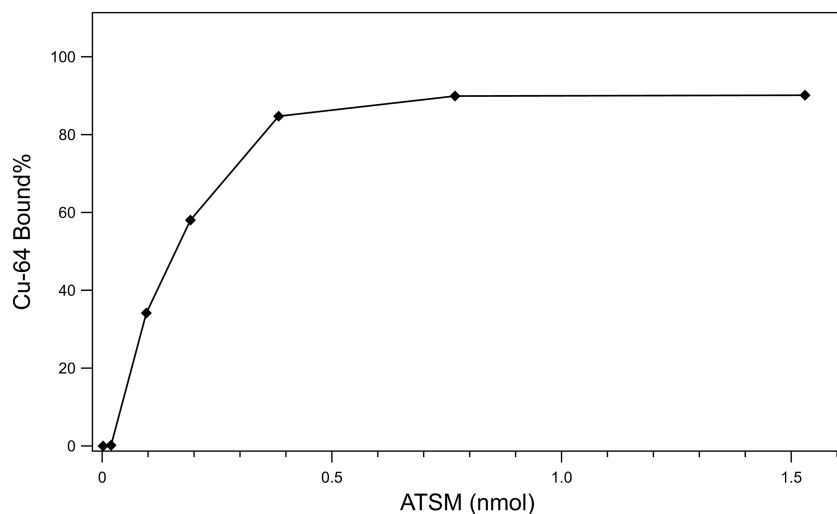
FIGURE 6 Titration plot showing bound Cu as a function of ATSM chelator amount
