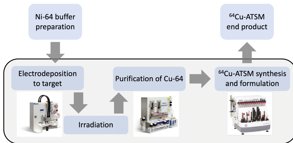
FIGURE 1 Overview of the synthesis workflow from cyclotron to finished product
