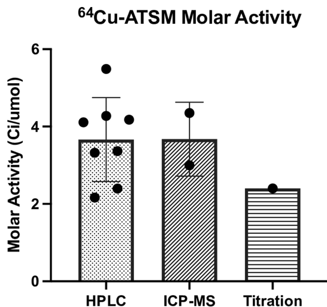
FIGURE 4 Comparison of the molar activity measured from HPLC, ICP-MS, and titration
