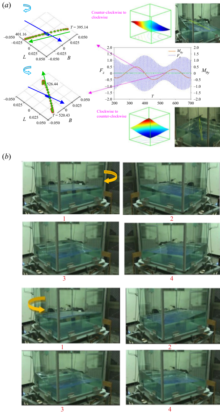
Figure 12. (a) Single-directional waves always occur at the peak and trough of F_z -envelope (snapshots: arrow sign in blue colour indicates the tank motion direction, arrow sign in green colour indicates the trajectory of mass volume centre); (b) snapshots of clockwise swirling waves (upper subplot in sequential order 1→2→3→4) and counterclockwise swirling waves (lower subplot in sequential order 1→2→3→4).
