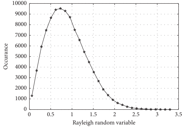
FIGURE 8: Rayleigh fading.
