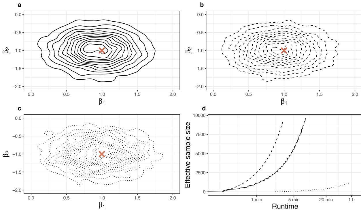
Figure 3. The joint posterior distribution of \beta in the bivariate linear model obtained using AMIS-INLA (—, a), IS-INLA (---, b), MCMC-INLA (⋯⋯, c), and the running effective sample size (d) of the respective methods. The (X) denotes the values of \beta chosen for the simulation of data.
