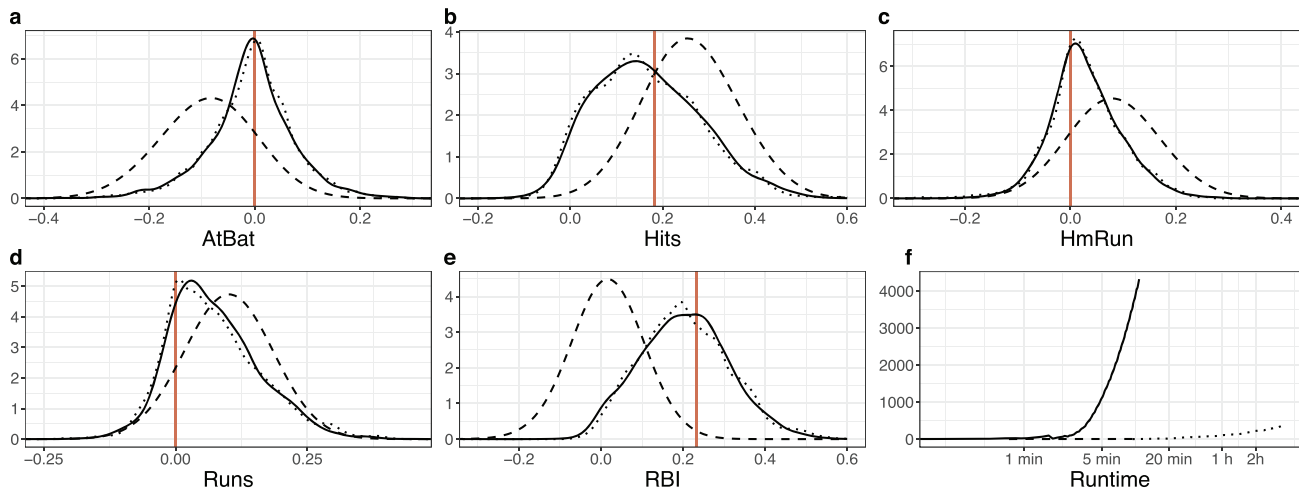
Figure 4. Approximate posterior marginals of the coefficients of the Bayesian Lasso model (a–e) fitted with AMIS-INLA (—), IS-INLA (---) and MCMC-INLA (⋯⋯), and the Lasso estimates of the coefficients (|). The running effective sample sizes of the respective methods are shown in (f), where runtimes are presented in a logarithmic scale.
