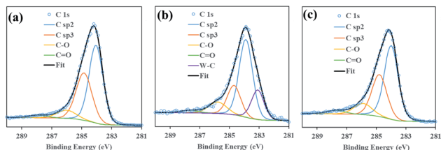
Fig. 3 High resolution C 1s XPS spectra of (a) DLC, (b) 10WDLC and (c) 10AgDLC.
