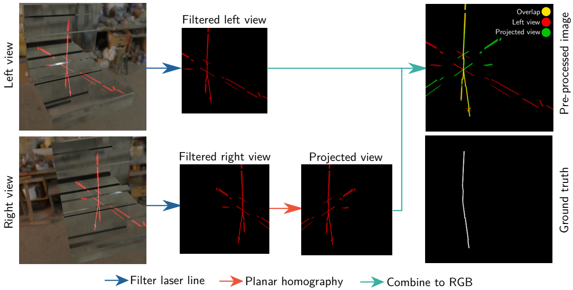
Figure 10: The planar homography preprocessing requires a filtered view of the laser from two cameras. One of the filtered views is then projected using a planar homography, such that when the two views are combined, the true laser line will overlap while many spurious reflections will not.
