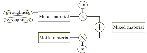
Figure 7: Mixed material generation. A Luxcore metal material is defined by the roughness in the perpendicular directions u and v . The metal material is mixed with a matte material with a mix factor m .
