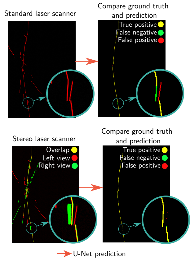
Figure 15: Specular reflection ambiguity. Sharp specular reflections may have a similar appearance as the true laser line. In certain cases, the single camera scanner incorrectly chooses the false reflection, while the stereo camera scanner chooses the true line since they are overlapping from both cameras.
