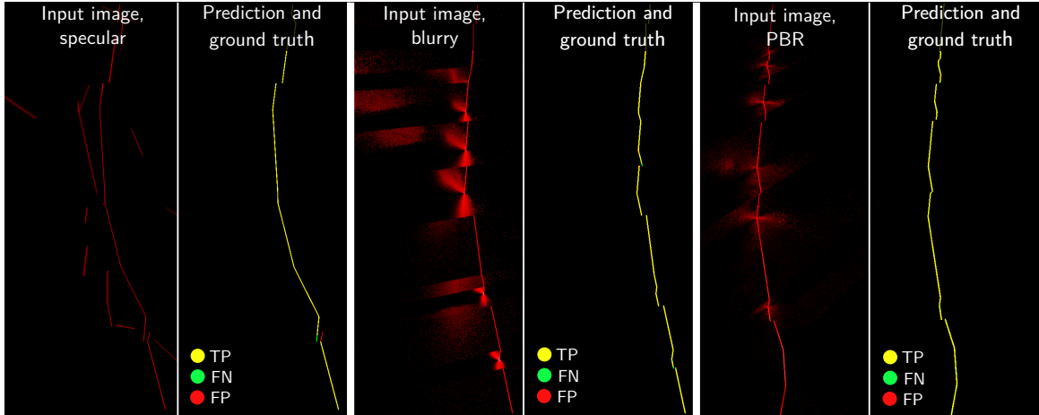
(a) Single camera laser scanner results.
