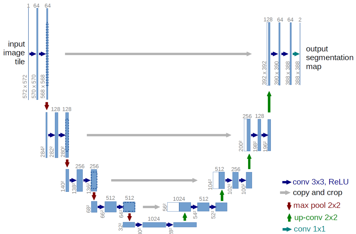
Figure 3: U-Net architecture (Ronneberger et al., 2015). The blue boxes show the feature maps with the number of channels denoted on top. The width and height of the feature maps used in the original paper are shown to the left of each blue box, however this depends on the input image size.
