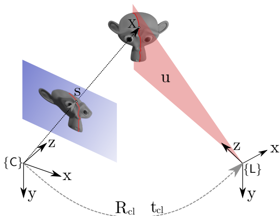
Figure 1: Laser scanner geometry. The camera frame is shown to the left and the laser frame to the right. The normalized image plane is drawn in front of the camera.
