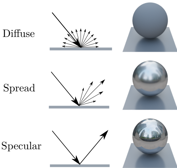
Figure 2: Basic reflection models. Diffuse reflections emit light equally in all directions, spread reflections emit in a set of directions, while specular reflections emit light in a single direction.
