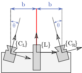
Figure 9: Stereo laser scanner
