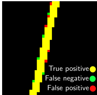
Figure 13: Imperfect edge detection. The U-Net prediction of the laser line is often incorrect at the edges of the laser line.
