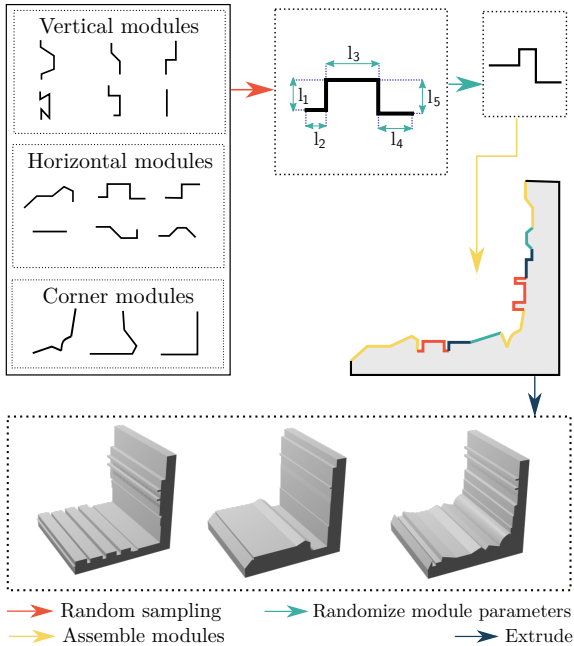
Figure 5: Mesh generation pipeline. A set of predefined modules are randomly sampled and the individual line lengths of the modules are randomized. One corner module, five vertical and five horizontal modules are assembled and extruded to a mesh.
