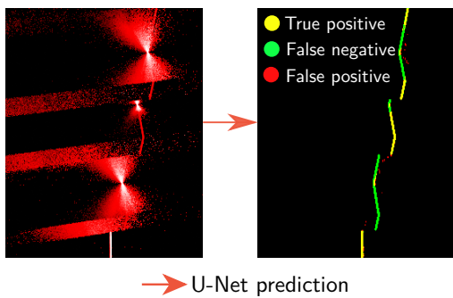
Figure 14: Strong blurry reflections may overlap the true scan line, such that it is not visible among the strong reflections.
