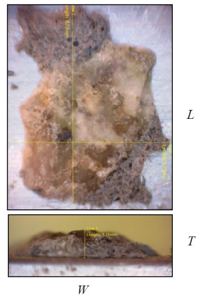
Figure 9 –Top: Scaled material after sieving. Bottom, left: Flakes mounted on a hollow steel bar with quadratic cross section by double-sided tape. Bottom, right: Digital photos taken perpendicular and parallel to the surface of the steel bar made it possible to determine thickness ( T ), length ( L ) and width ( W ) of the individual flakes accurately. (Illustrations from [14]).
