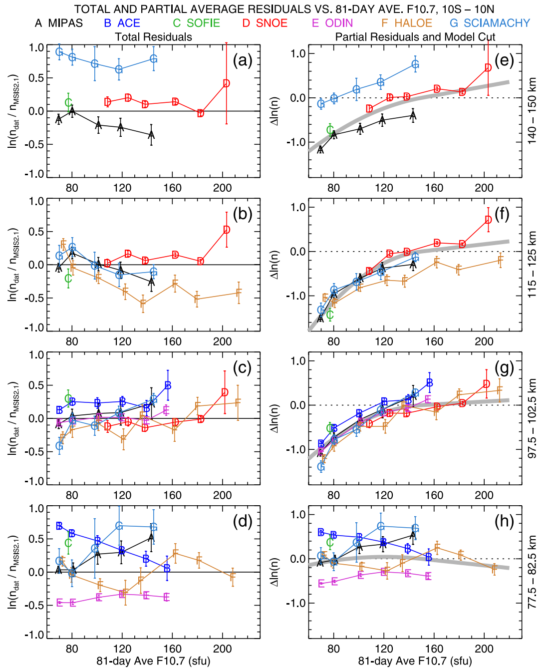
Figure 9. Same analysis as Figure 7, but as a function of \overline{F}_{10.7} (the 81-day average of the daily F_{10.7} ), near the equator ( 10^{\circ}\text{S} – 10^{\circ}\text{N} ), and including data from all times of the year. The \overline{F}_{10.7} bins are 65–75, 75–90, 90–110, 110–130, 130–150, 150–170, 170–200, and 200–230 sfu. In panels (e–h) on the right, the partial residuals were calculated relative to MSIS 2.1 with the \overline{F}_{10.7} terms and the coupled \overline{F}_{10.7} -latitude terms turned off. The thick gray curve shows the \overline{F}_{10.7} variation of the model referenced to the model value at \overline{F}_{10.7} = 150 sfu.
