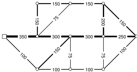
Figure 3. Fictitious example network, with pipe diameter labels.
