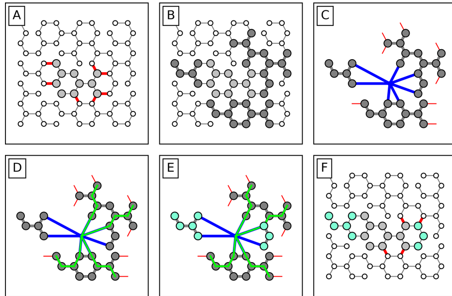
Figure 10. Conceptual steps made by the hybrid variator to reduce the number of boundaries of a specific DMA by assimilation certain nearby nodes. The individual steps are explained in more detail in the text.
