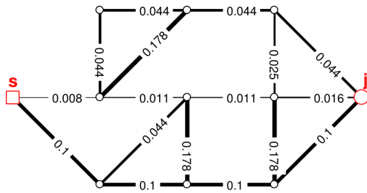
Figure 4. Network represented as weighted graph with edge weights w_i = L_i/D_i^2 .
