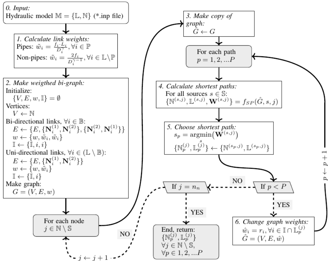
Figure 2. Flow chart with suggested algorithm for identifying principal paths.
