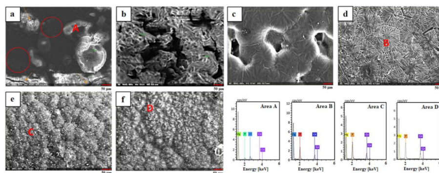
Figure 5. FESEM micrographs of (a,b) uncoated Mg, (c) PCL/CS, (d) PCL/CS/2ZnO, (e) PCL/CS/4ZnO, and (f) PCL/CS/6ZnO composite-coated Mg specimens and EDX analysis of Area A, B, C, and D.
