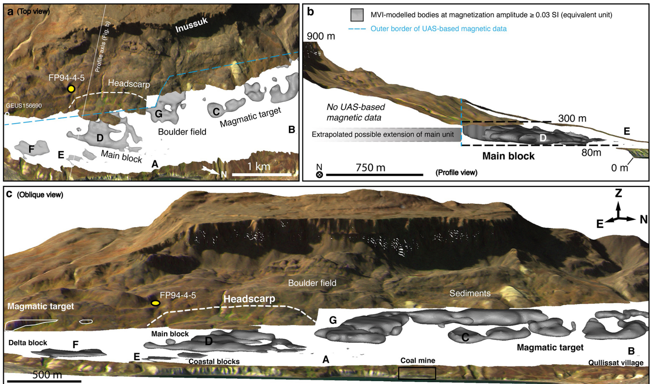
Figure 13. Combined plots of surface topography (PlanetScope mosaic fused with ArcticDEM) and larger magnetization amplitudes ( \geq 0.03 SI) in the subsurface from the MVI model: (a) top view of survey area; (b) side view cross section facing north – dashed lines indicate the maximum extension of the intrusive body; (c) oblique view from the east. In all three views the surface model is removed for areas where the magmatic body is present at the surface (compare Figs. 12a, 14a). A possible extension of the target unit is sketched next to the main block, anomaly D.
