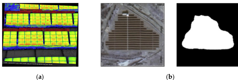
Figure 3. Examples of detection types for the detection of PV systems using aerial imagery: (a) boxes Reprinted with permission from ref. [61]. Copyright 2020 Copyright Elsevier; (b) mask [57].
