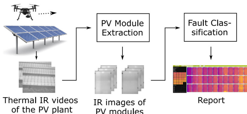
Figure 4. Overview of a tool for semi-automatic inspection of large-scale PV plants using IRT videos acquired by a UAV [88].
