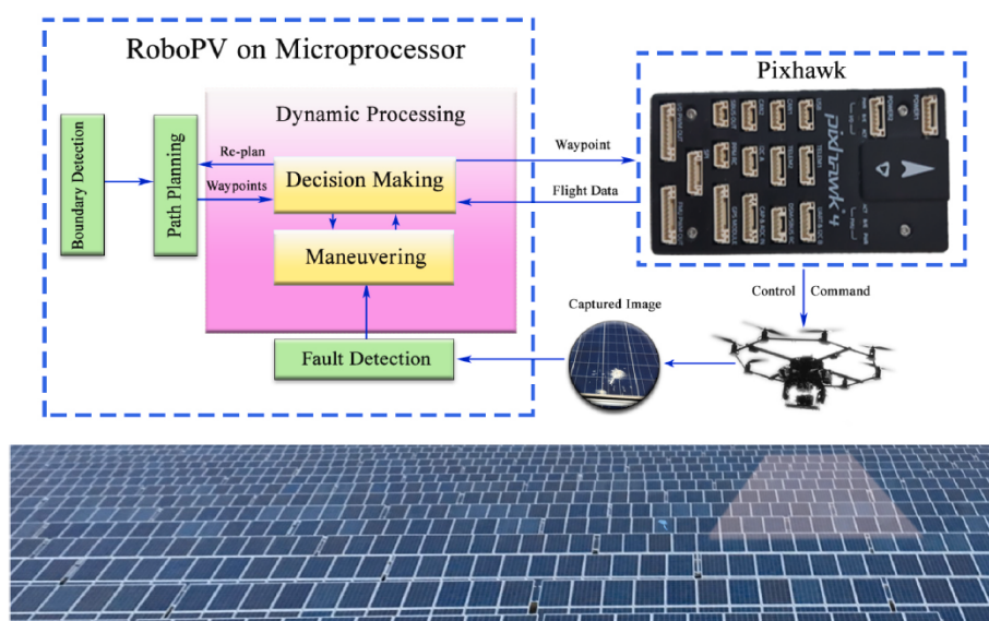
Figure 5. Overview of the on-board software package RoboPV, developed to perform the autonomous aerial monitoring of large-scale PV plants using UAVs [51].
