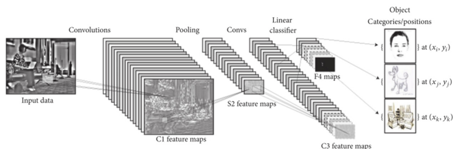
Figure 1. Example architecture of a CNN for an object detection task [36].
