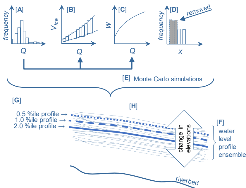
Figure 20. Adjustment in the boundary condition frequency distribution within the stochastic modelling framework when considering mitigation options, such as artificially breaking the ice cover to hinder ice-jam lodgments; explanations for each subfigure are provided in the main text (drawn by the first author).
