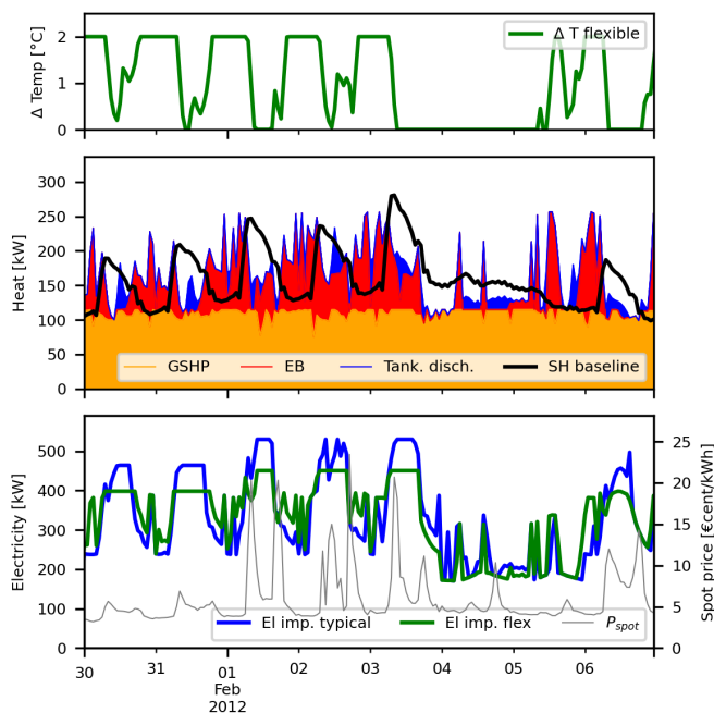
Figure 2: Operational details of the GSHP-flex case, week 5.
