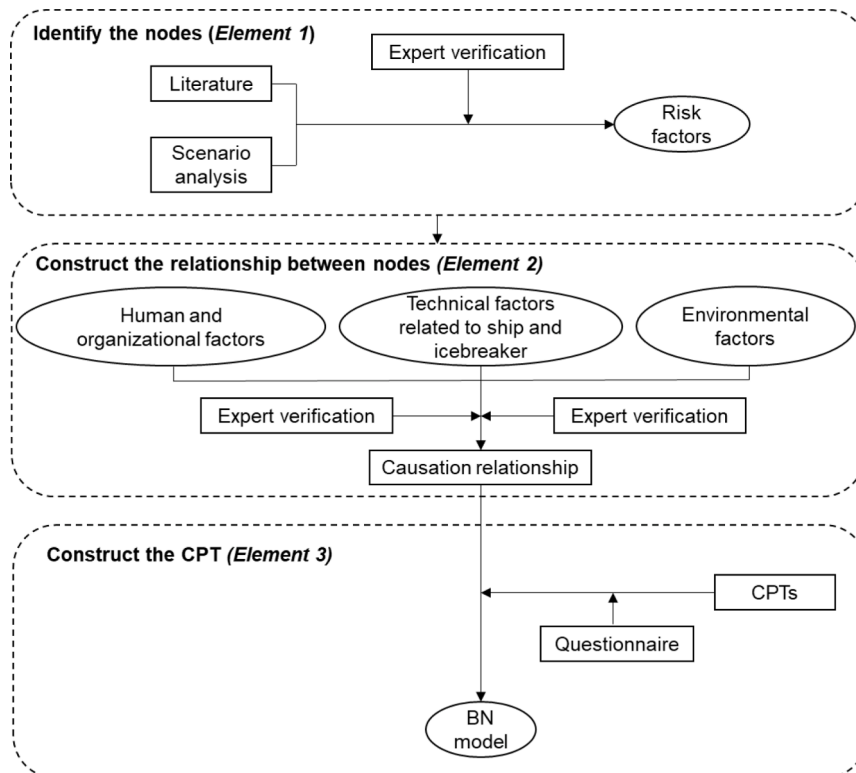
Fig. 1. BN development framework for ship besetting in ice in convoy operations.
