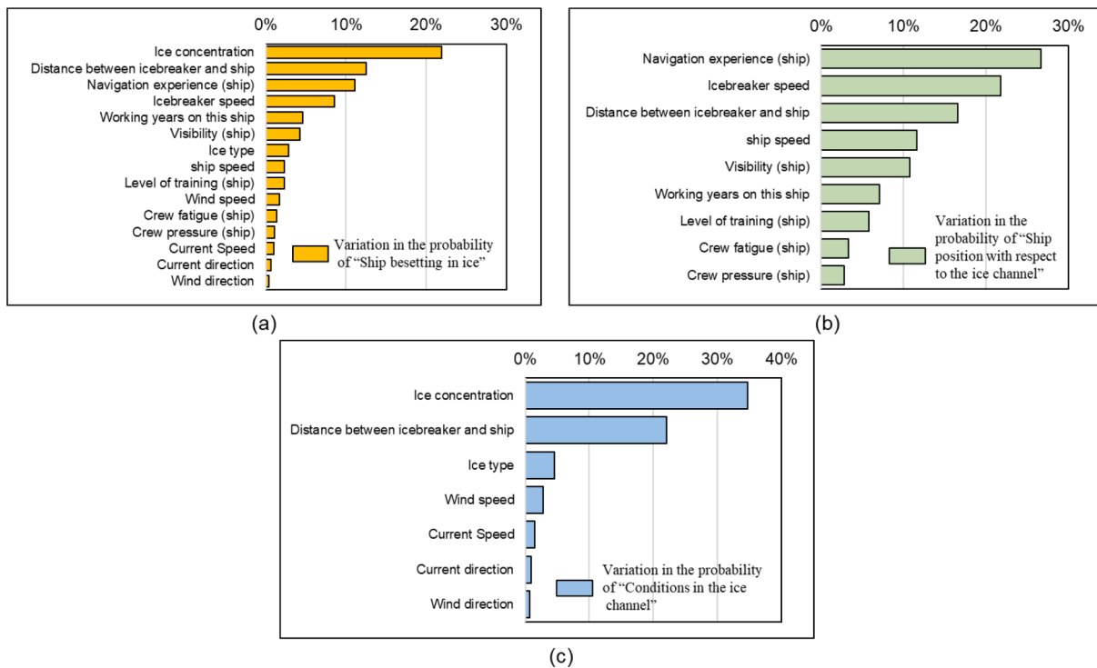
Fig. 9. Sensitivity of each basic node to the target node. (a) For the target node ‘Ship besetting in ice’. (b) For the target node ‘Ship position with respect to the ice channel’. (c) For the target node ‘Conditions in the ice channel’.
