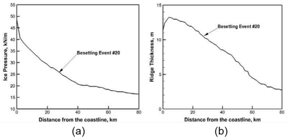
Fig. 7. (a) Ice pressure versus distance from the coastline, (b) Ridge thickness versus distance from the coastline [17].
