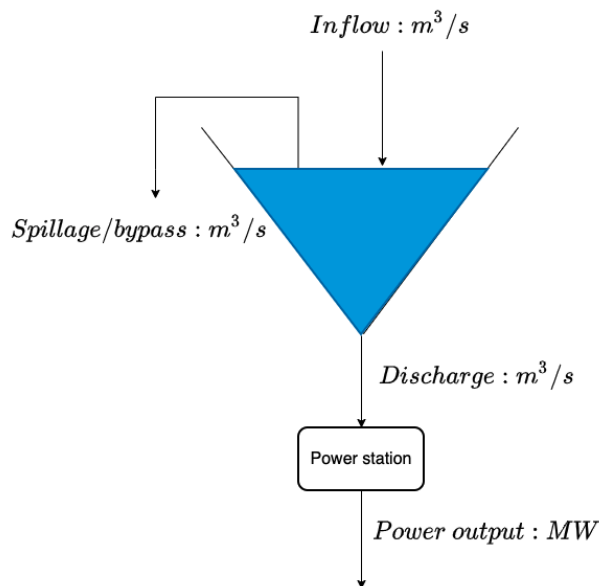
Figure 3.3: Representation of discharge, spillage/bypass and inflow in hydropower production
