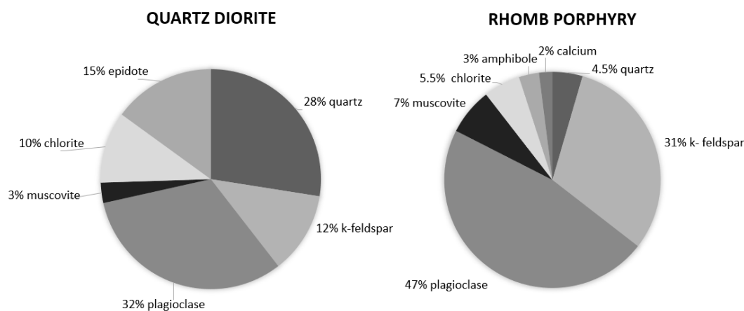
Figure 1. Mineral composition, in percent, of quartz diorite and rhomb porphyry.
