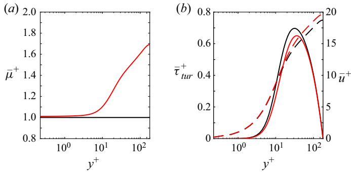
Figure 1. Mean viscosity, Reynolds shear stress and velocity profiles: (a) \bar{\mu}^+ and (b) \bar{\tau}_{ur}^+ , \bar{u}^+ . In (a), \mu_\infty/\mu_0 = 1 \times 10^{-3} , \mu_0^+ \approx 1.782 , \Lambda^+ = 0.1 and \alpha is set to 0.8 and to 1 for cases P180 and N180, respectively. In (b), profiles corresponding to \bar{\tau}_{ur}^+ and \bar{u}^+ are indicated by the line styles ‘—’ and ‘- -’, respectively. Line colours as explained in table 1.
