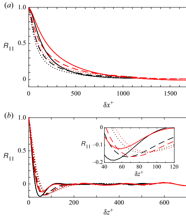
Figure 18. Normalized two-point correlation R_{11} with: (a) streamwise separation, \delta x^+ , and (b) spanwise separation, \delta z^+ . Line styles ‘—’, ‘---’ and ‘···’ are used to identify correlations at y^+ \approx 5, 30 and 50 , respectively. Line colours as explained in table 1.
