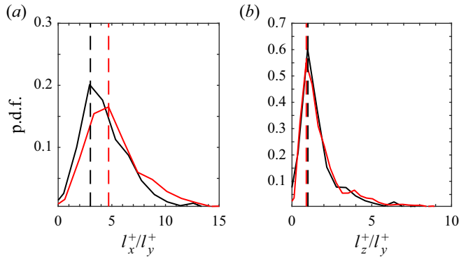
Figure 14. The p.d.f. of the bounding boxes' aspect ratios: (a) l_x^+/l_y^+ and (b) l_z^+/l_y^+ corresponding to the wall-attached structures, y_{min}/h \gtrsim 20/h^+ , confined to the viscous wall region, y_{max}/h \lesssim 50/h^+ . Dashed vertical lines mark the approximate peak values of the p.d.f. Line colours as explained in table 1.
