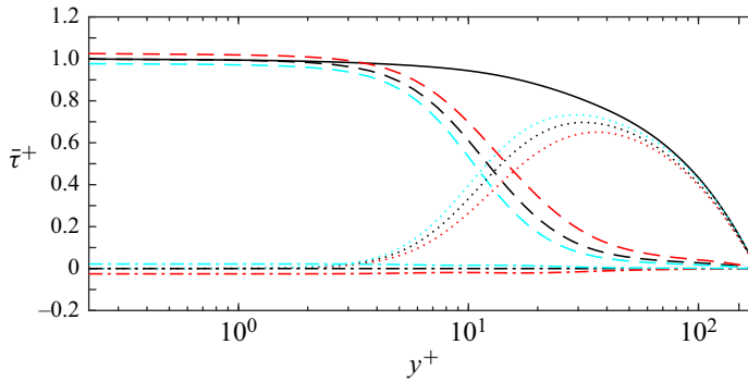
FIGURE 9. Mean shear stress budget. Line styles ‘—’, ‘- - -’, ‘...’ and ‘- . -’ are used to identify \bar{\tau}^+ , \bar{\tau}_{vis}^+ , \bar{\tau}_{tur}^+ and \bar{\tau}_{GN}^+ , respectively. Profiles corresponding to P180, N180 and D180 are identified by red, black and cyan colours, respectively.
