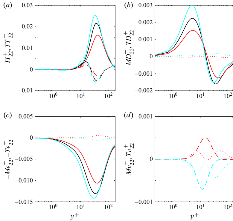
FIGURE 22. Contributions to T_{22}^+ and -\epsilon_{22}^+ in budget B_{22}^+ : (a) line styles ‘—’ and ‘- - -’ are used for \Pi_{22}^+ and TT_{22}^+ ; (b) line styles ‘—’ and ‘...’ are used for MD_{22}^+ and TD_{22}^+ ; (c) line styles ‘—’ and ‘...’ are used for -M\epsilon_{22}^+ and -T\epsilon_{22}^+ ; and (d) line styles ‘- - -’ and ‘...’ are used for Mv_{22}^+ and Tv_{22}^+ . Profiles corresponding to P180, N180 and D180 are identified by red, black and cyan colours, respectively.
