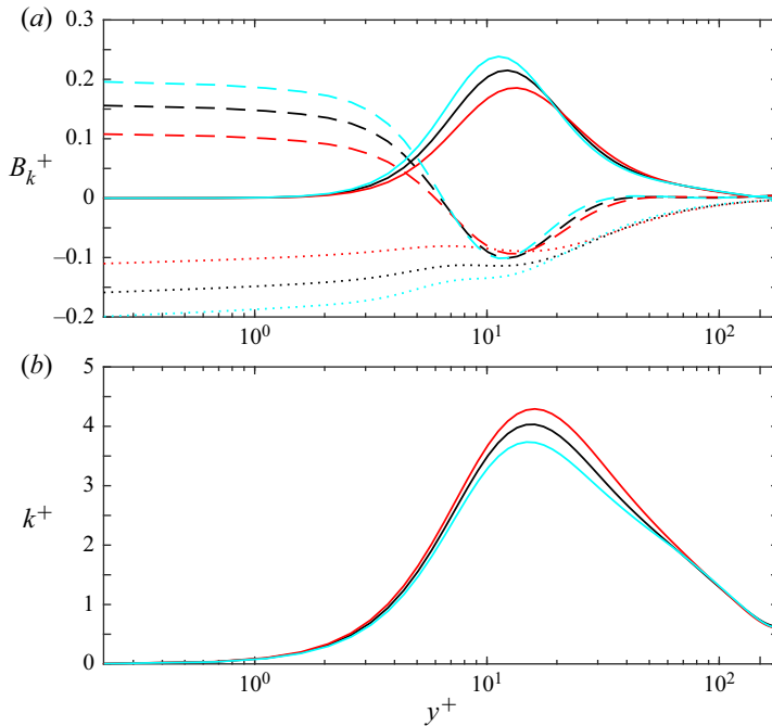
FIGURE 13. Plots of (a) B_k^+ and (b) k^+ . In panel (a), the line styles ‘—’, ‘- - -’ and ‘· · ·’ are used to identify P_k^+ , T_k^+ and -\epsilon_k^+ , respectively. Profiles corresponding to P180, N180 and D180 are identified by red, black and cyan colours, respectively.
