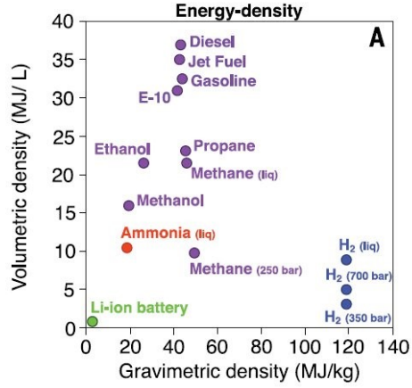
Figure 3.12: Energy density comparison among some fuels [44]
