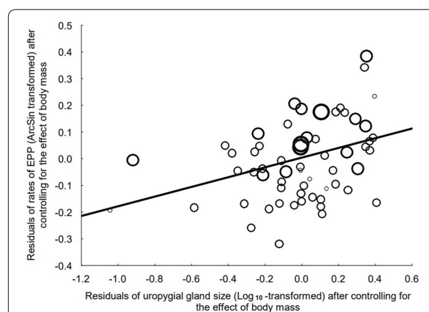
Fig. 1 Association between residuals of rate of extra pair paternity and volume of the uropygial gland of the 60 avian species considered in the study after controlling for the effect of body mass. Line is the regression line and size of circles are proportional to \log_{10} -transformed sample size used to estimate extra pair paternity in each species
