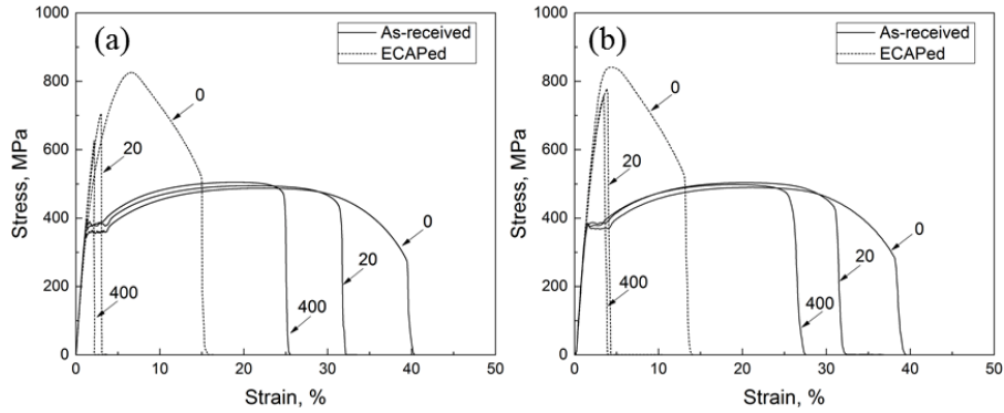
Fig. 3. Stress-strain diagrams of the as-received and ECAPed specimens before and after hydrogen charging at low (a) and high (b) strain rate.
