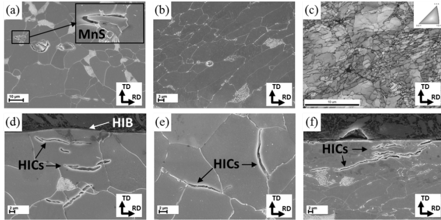
Fig. 1. SEM images (a, b, d-f) and inverse pole figure (IPF) colored orientation map obtained by EBSD from the microstructure of the as-received (a, d, e) and the ECAPed (b, c, f) specimens of the low-alloy steel grade 09G2S before (a-c) and after (d-f) cathodic hydrogen charging
