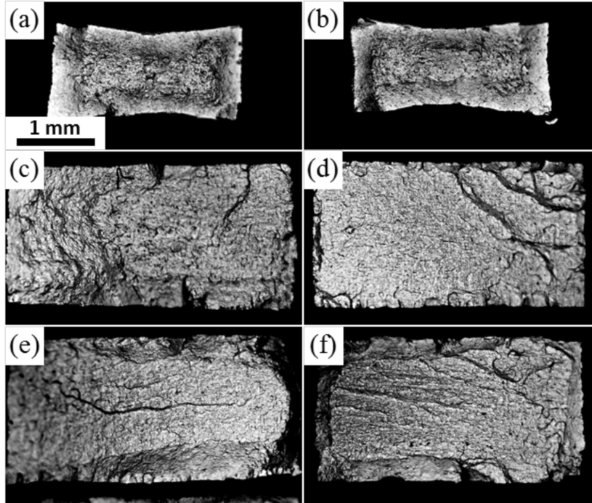
Fig. 6. Full-scale views of the fracture surfaces of the ECAPed specimens of the low-alloy steel grade 09G2S tested at 5 (a, c, e) and 50 mm/min (b, d, f) traverse velocity in the hydrogen free state (a, b) and after hydrogen charging at 20 (c, d) and 400 mA/cm 2 (e, f). Backscattering electron contrast images obtained by SEM.
