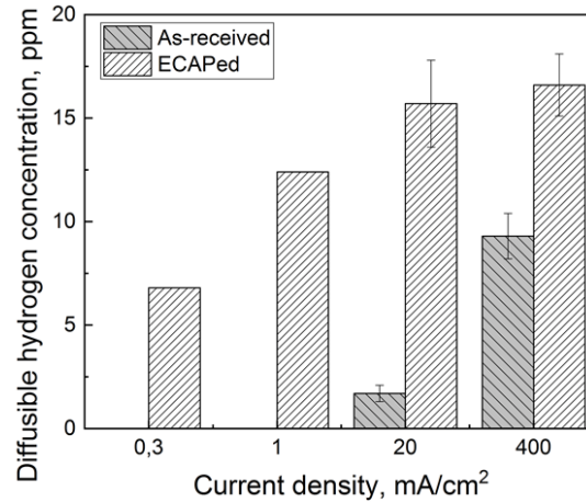
Fig. 2. Effect of cathodic hydrogen charging current density on the diffusible hydrogen concentration in the as-received and ECAPed low-alloy steel 09G2S.
