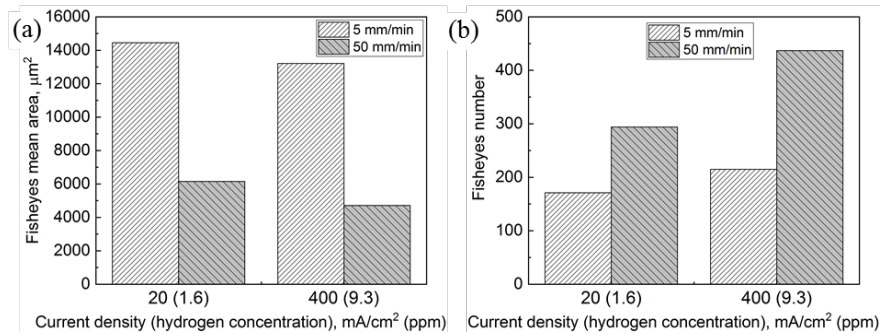
Fig. 8. Effect of cathodic hydrogen charging current density (diffusible hydrogen concentration) and strain rate on the mean area (a) and number (b) of fisheyes in the fracture surfaces of the hydrogen charged as-received specimens of the low-alloy steel grade 09G2S.
