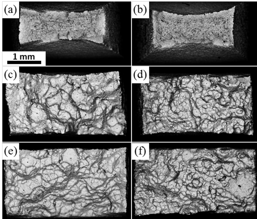
Fig. 5. Full-scale views of the fracture surfaces of the as-received specimens of the low-alloy steel grade 09G2S tested at 5 (a, c, e) and 50 mm/min (b, d, f) traverse velocity in the hydrogen free state (a, b) and after hydrogen charging at 20 (c, d) and 400 mA/cm 2 (e, f). Backscattering electron contrast images obtained by SEM.
