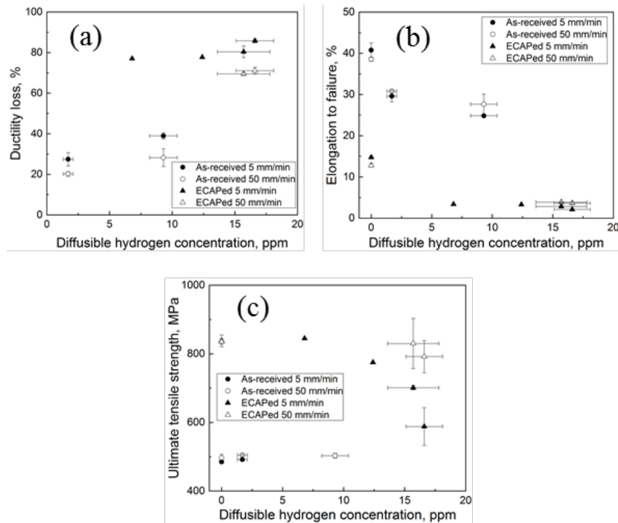
Fig. 4. Effect of the diffusible hydrogen concentration on the ductility loss (a), elongation to failure (b) and ultimate tensile strength (c) of the as-received and ECAPed specimens at low and high strain rate of tensile testing.
