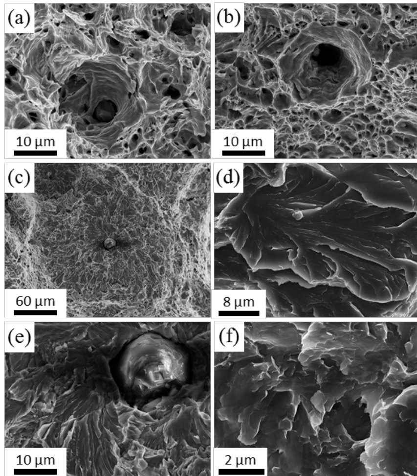
Fig. 7. SEM images demonstrating characteristic features of the fracture surfaces of the as-received (a-c) and ECAPed (d-f) specimens tested before (a, d) and after (b, c, e, f) hydrogen charging: (a, d) – dimpled relief, (b) – fisheye, (c) – fisheye’s quasi-cleavage, (e) – true cleavage, (f) – tearing morphology.
