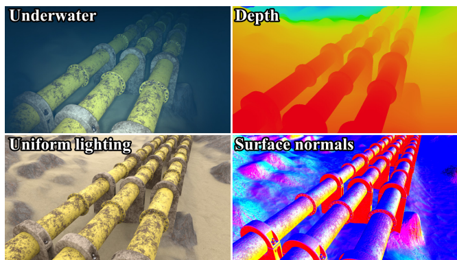
Figure 1. The image types contained in the initial version of the VAROS underwater dataset: underwater images and corresponding images with uniform lighting and no water, as well as pixel-accurate surface normal and depth maps.
