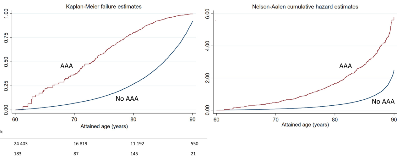
Figure 1 Kaplan-Meier failure plot and Nelson-Aalen cumulative hazard estimates in subgroups defined by AAA (no, yes). AAA, abdominal aortic aneurysm.
