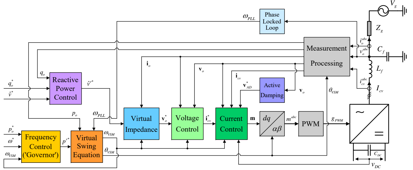
Fig. 1. Block diagram of the applied VSM-based control strategy for power-controlled HVDC terminal providing virtual inertia.
