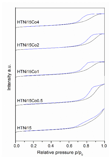
Fig. S1. Nitrogen sorption isotherms for the calcined catalysts
