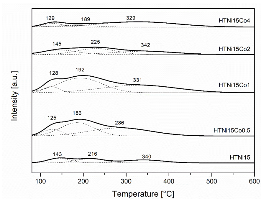
Fig. S2. CO 2 -TPD profiles for the reduced hydrotalcite-derived catalysts
