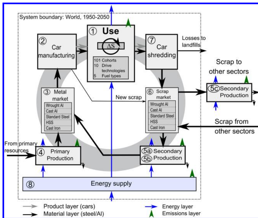
Figure 1. System definition. The model time runs from 1950 to 2010 with historical data and from 2011 to 2050 with scenario data. Car flows and stocks were divided into ten drive technologies. The model distinguishes cast iron, standard steel, high strength steel, cast aluminum, and wrought aluminum. Six energy carriers were considered: gasoline, diesel, coal, electricity, natural gas, and hydrogen.
