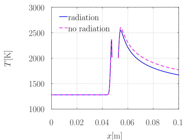
Fig. 8. Comparison of temperature profiles along the centerline with and without gas-to-gas radiation model.
