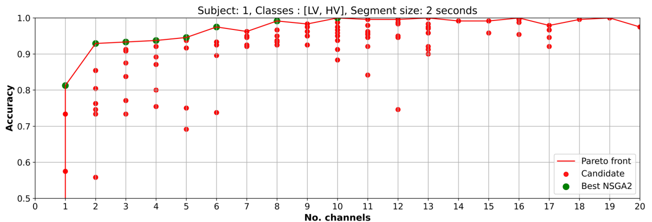
Figure 7. Optimized EEG channel selection results for low and high valence classification using EEGNet and data from subject 1.
