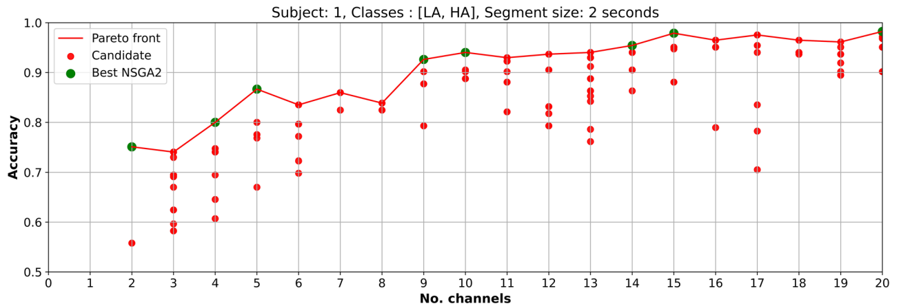
Figure 6. Optimized EEG channel selection results for low and high arousal classification using EEGNet and data from subject 1.
